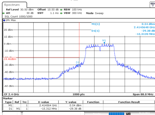
802.11g_2412MHz
