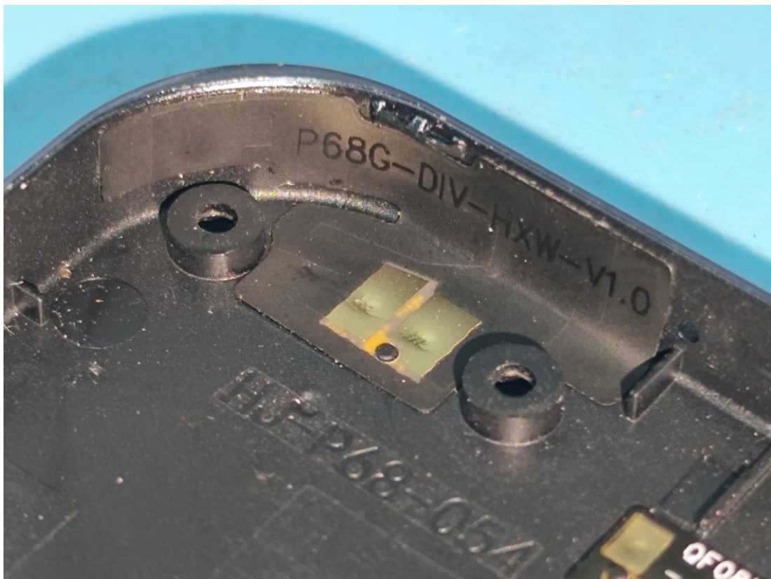
DIV Antenna
