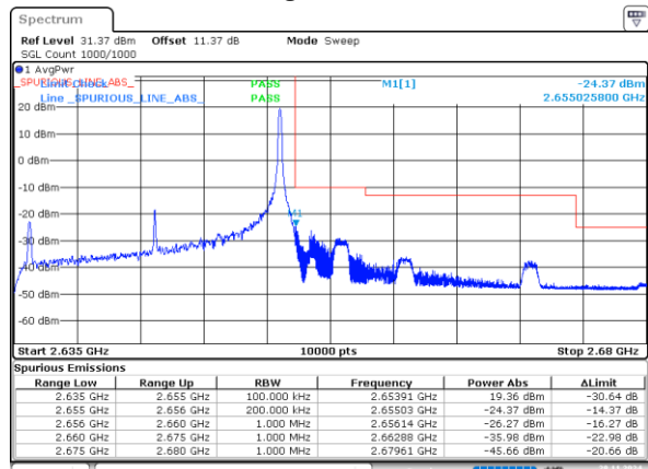
20MHz_High_16QAM_1@99
