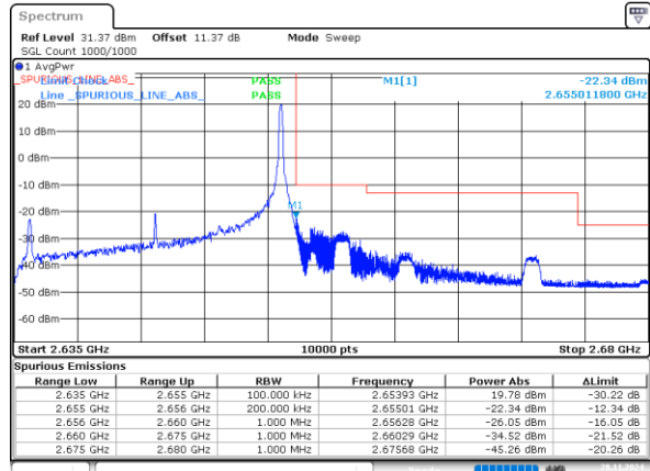
20MHz_High_QPSK_1@99
