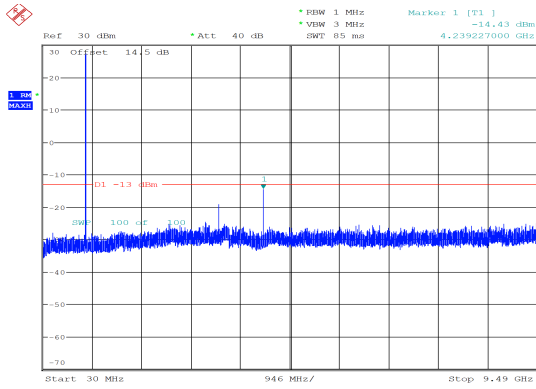
1.4MHz_High_QPSK_1@0 -14.43 dBm
