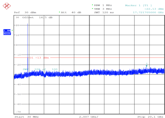
10MHz_Low_QPSK_1@49 -22.13 dBm
