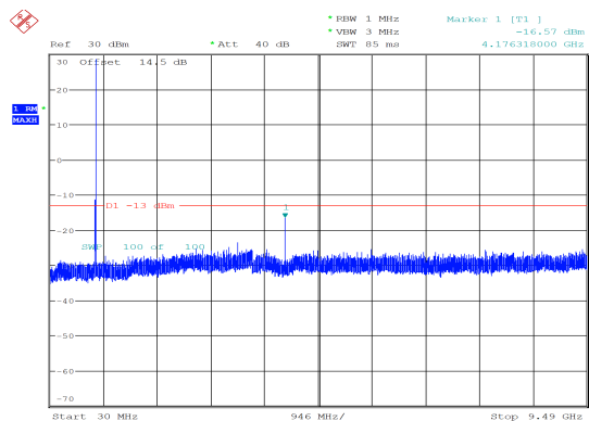
3MHz_Middle_QPSK_1@0 -16.57 dBm
