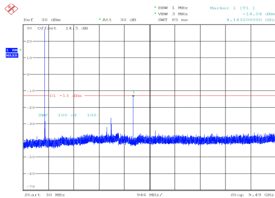
5MHz_Low_QPSK_1@24 -14.04 dBm
