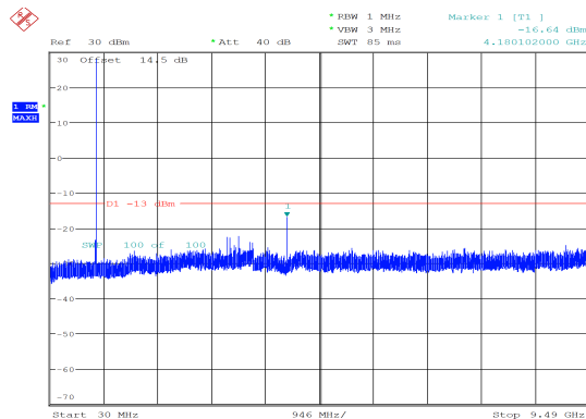
1.4MHz_Middle_QPSK_1@0 -16.64 dBm
