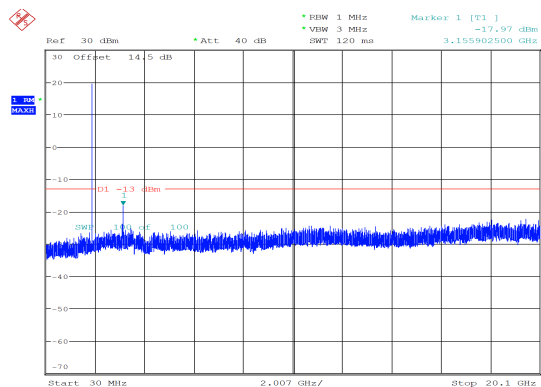
3MHz_High_QPSK_1@14 -17.97 dBm
