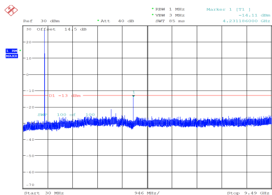
3MHz_High_QPSK_1@0 -14.11 dBm
