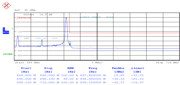
10MHz_High_QPSK_1@49
