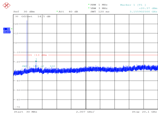
3MHz_High_QPSK_1@0 -20.37 dBm
