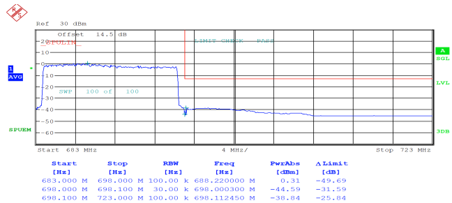
15MHz_High_QPSK_75@0
