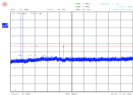
1.4MHz_Low_QPSK_1@0 -14.43 dBm
