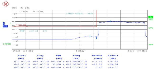
15MHz_Low_QPSK_75@0
