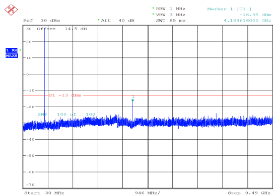
3MHz_Middle_QPSK_1@14 -16.95 dBm
