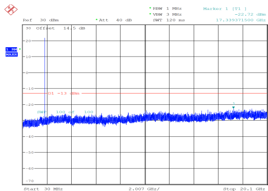
5MHz_Low_QPSK_1@0 -22.72 dBm
