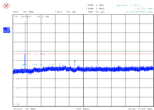
3MHz_Middle_QPSK_15@0 -22.29 dBm
