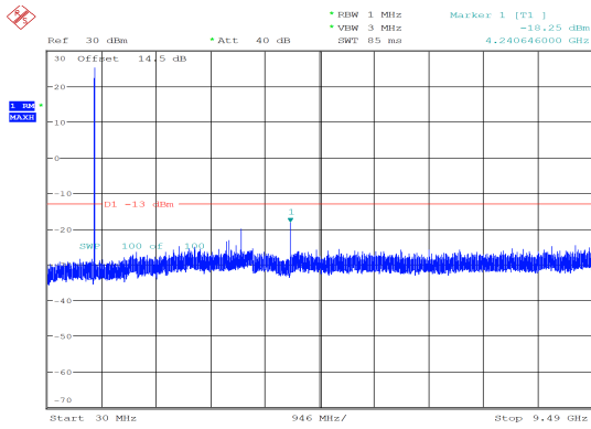
1.4MHz_High_QPSK_6@0 -18.25 dBm
