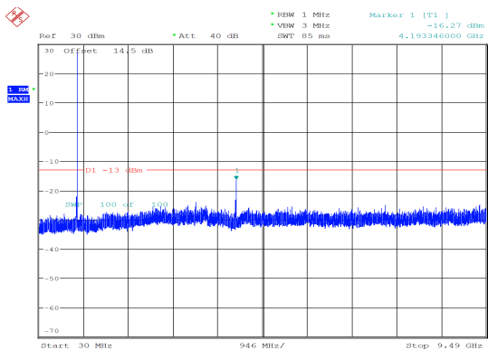
5MHz_Middle_QPSK_1@24 -16.27 dBm
