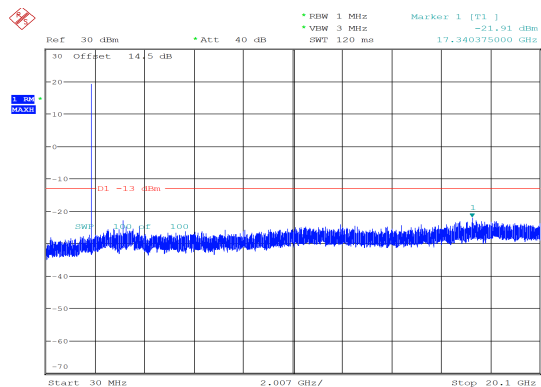
3MHz_Middle_QPSK_15@0 -21.91 dBm
