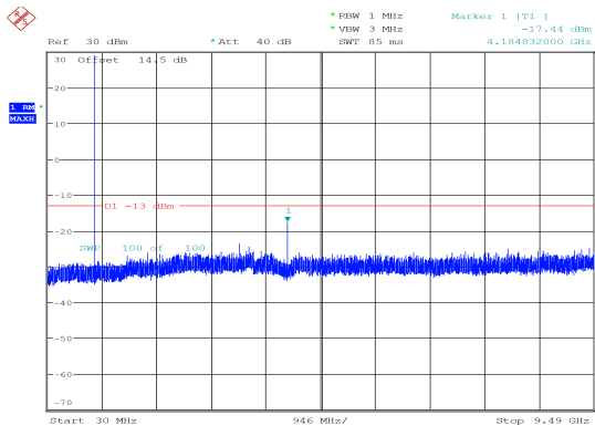
1.4MHz_Middle_QPSK_1@5 -17.44 dBm
