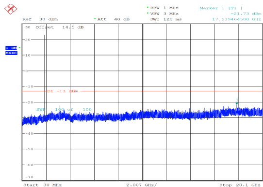
5MHz_Middle_QPSK_1@0 -21.73 dBm
