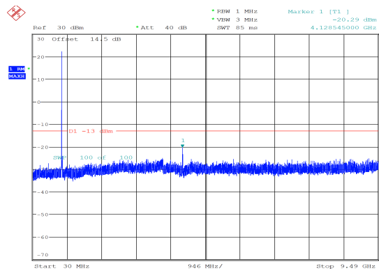
3MHz_Low_QPSK_15@0 -20.29 dBm
