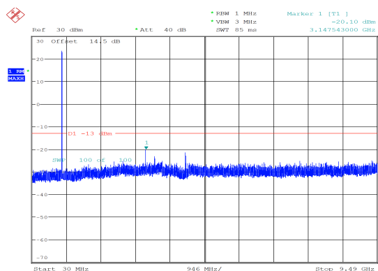
3MHz_High_QPSK_15@0 -20.10 dBm
