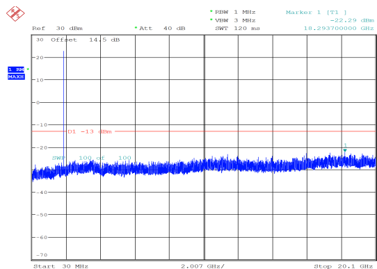
5MHz_Middle_QPSK_1@24 -22.29 dBm
