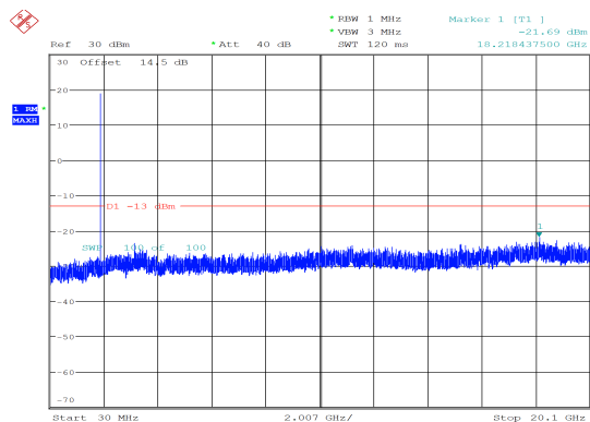
3MHz_High_QPSK_15@0 -21.69 dBm
