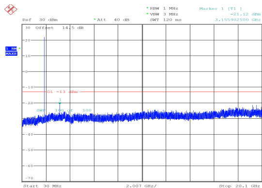
3MHz_Middle_QPSK_1@14 -21.12 dBm
