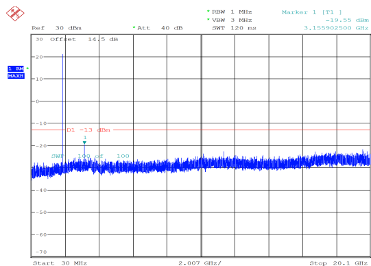
3MHz_Middle_QPSK_1@0 -19.55 dBm
