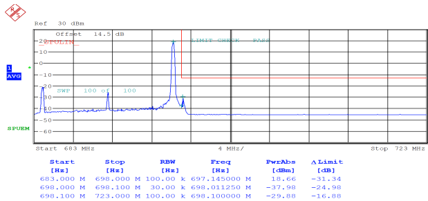
15MHz_High_QPSK_1@74
