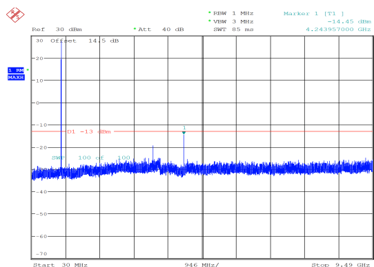
3MHz_High_QPSK_1@14 -14.45 dBm
