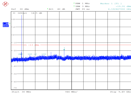
1.4MHz_Middle_QPSK_6@0 -19.91 dBm
