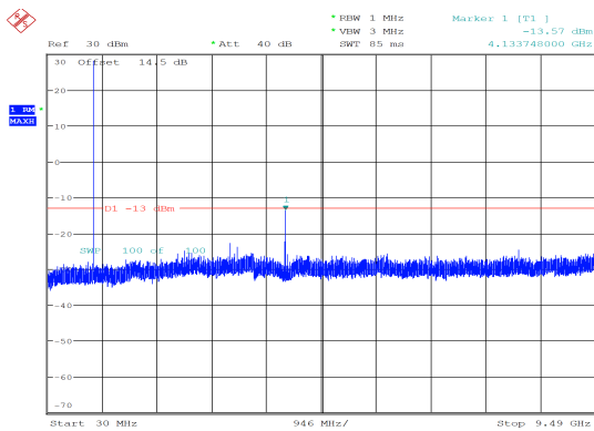
3MHz_Low_QPSK_1@14 -13.57 dBm
