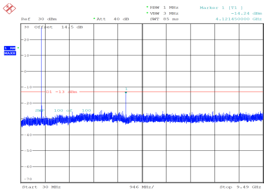
5MHz_Low_QPSK_1@0 -14.24 dBm
