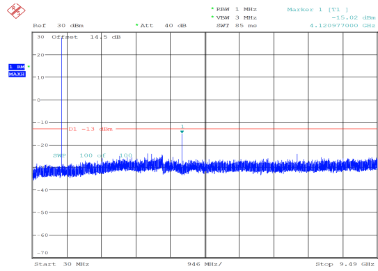
3MHz_Low_QPSK_1@0 -15.02 dBm
