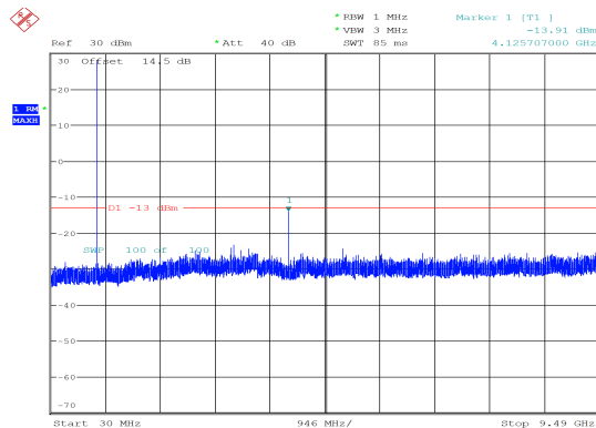
1.4MHz_Low_QPSK_1@5 -13.91 dBm
