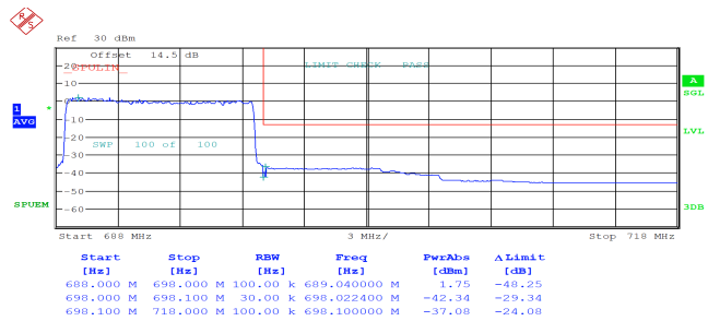
10MHz_High_QPSK_50@0
