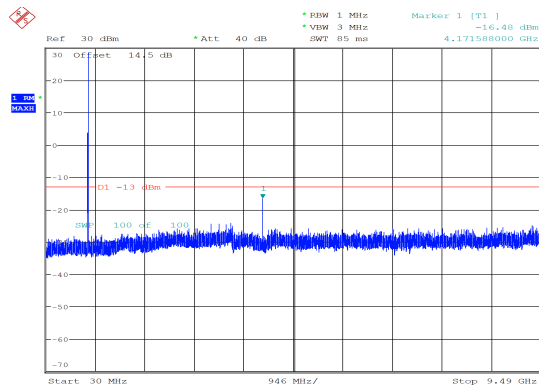
5MHz_Middle_QPSK_1@0 -16.48 dBm
