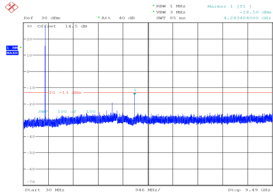
1.4MHz_High_QPSK_1@5 -14.59 dBm
