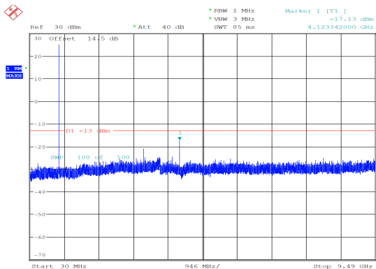
1.4MHz_Low_QPSK_6@0 -17.13 dBm
