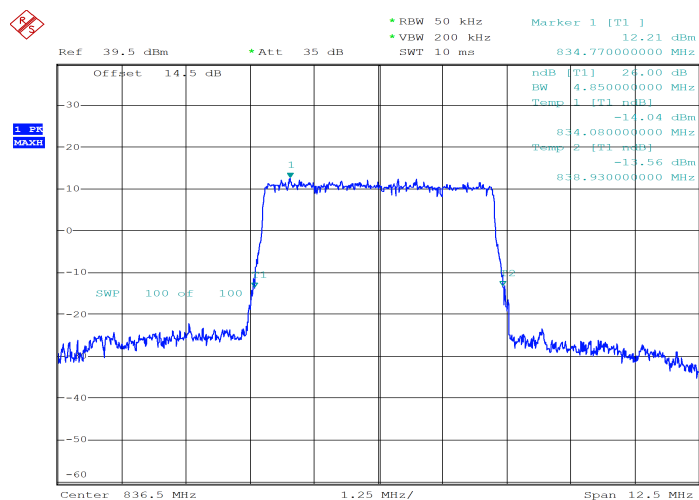
26dB Bandwidth 4.850MHz
