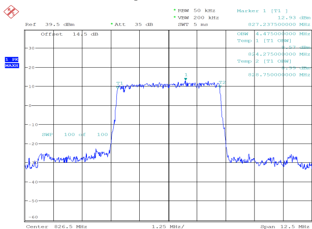
99% Occupied Bandwidth 4.475 MHz
