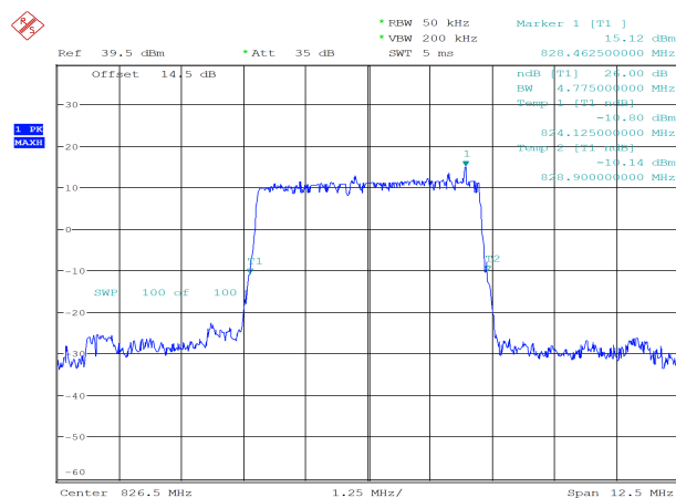
26dB Bandwidth 4.775MHz
