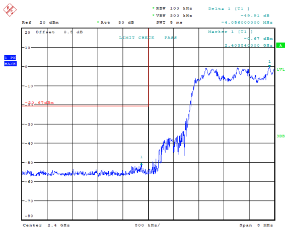
8DPSK_Hopping_Lower 49.91 dB
