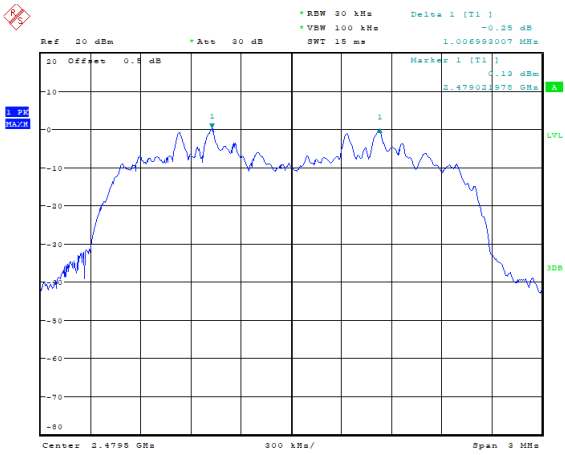
8DPSK_High 1.007 MHz
