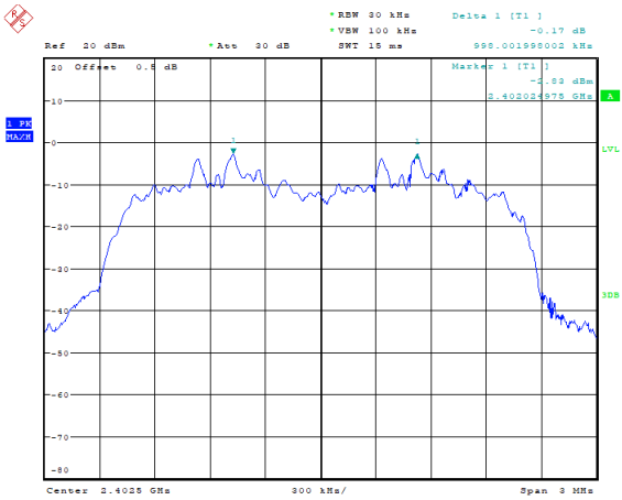
8DPSK_Low 0.998 MHz
