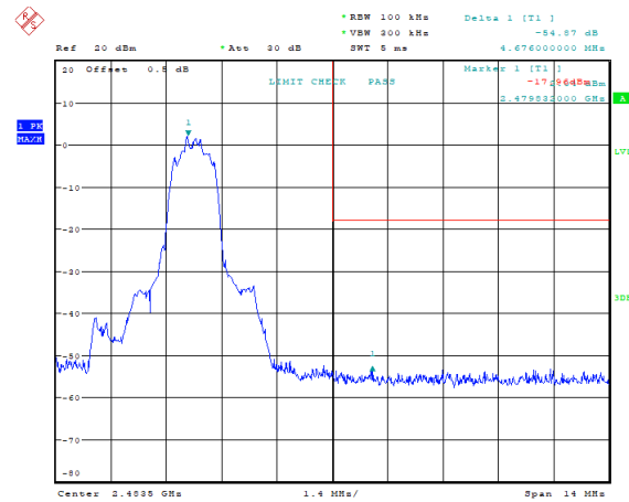
8DPSK_High 54.87 dB
