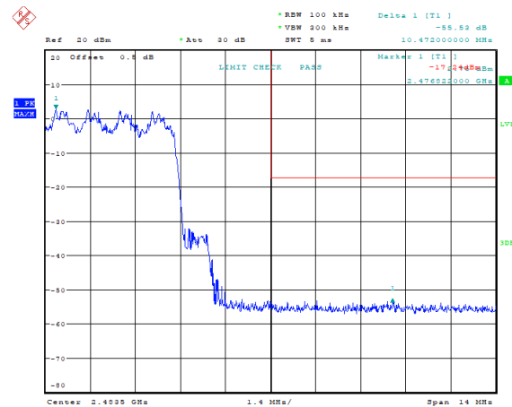
8DPSK_Hopping_Upper 55.53 dB
