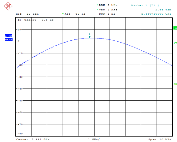
GFSK_Middle 2.56 dBm
