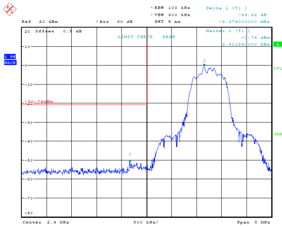
8DPSK_Low 49.22 dB
