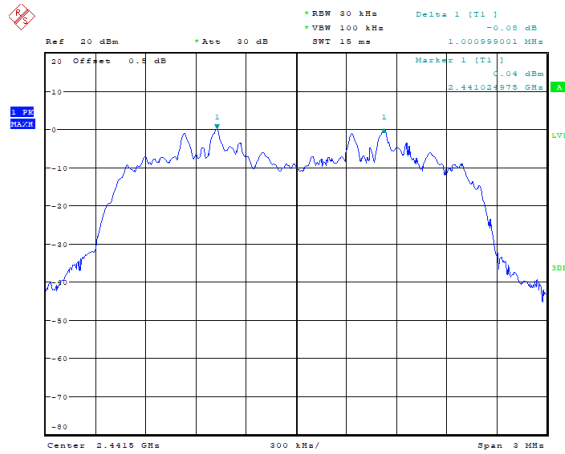
8DPSK_Middle 1.001 MHz
