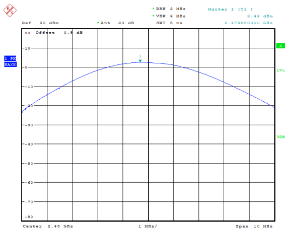
GFSK_High 2.43 dBm
