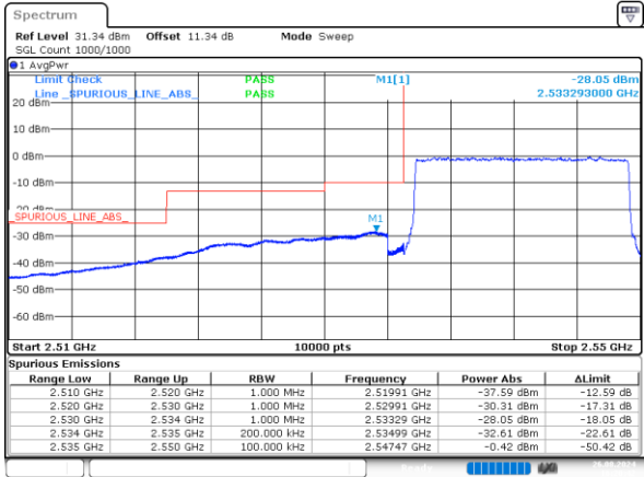
2_15MHz_Low_16QAM_75@0
