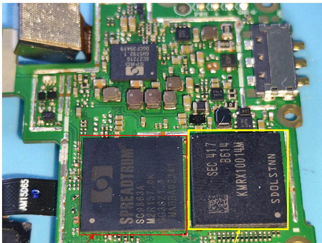
Main Chip
