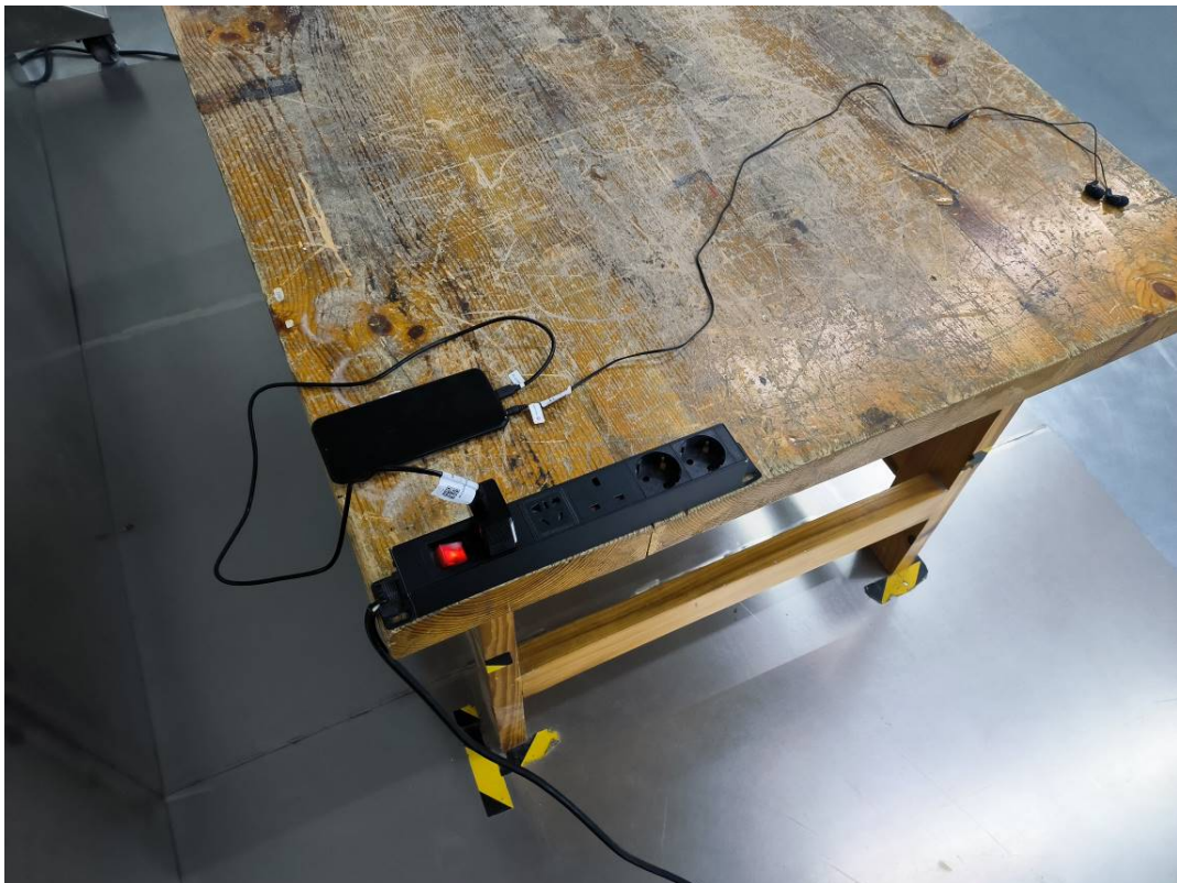
Conducted Emissions Side View Adapte 2#
