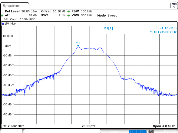
BLE_1M_Low_Channel_Reference Level
