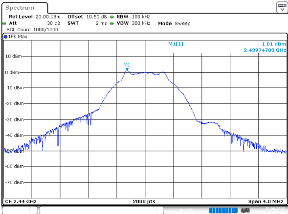
BLE_1M_Middle_Channel_Reference Level
