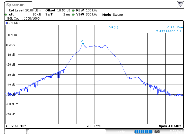
BLE_1M_High_Channel_Reference Level
