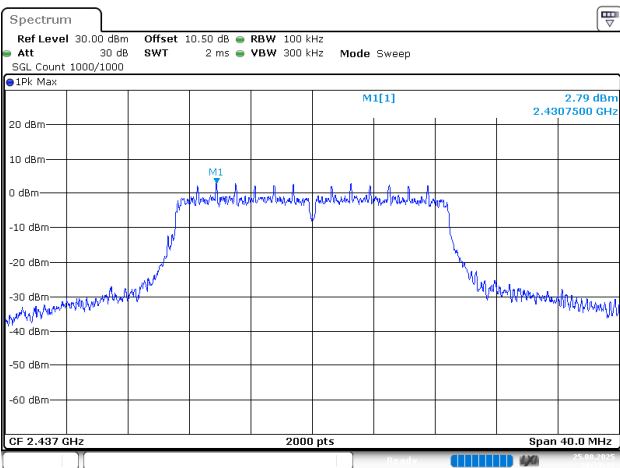
802.11n ht20_2437MHz_Reference Level
