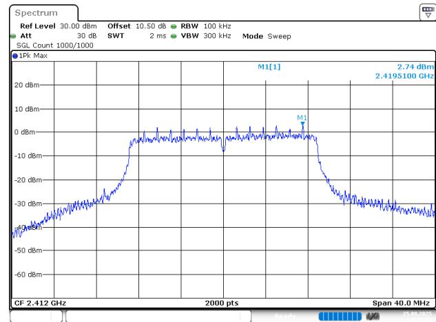
802.11n ht20_2412MHz_Reference Level
