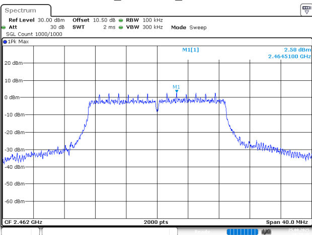
802.11n ht20_2462MHz_Reference Level
