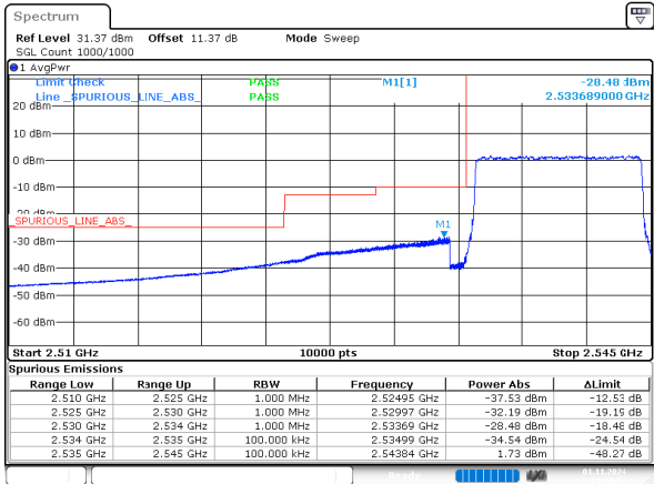
2_10MHz_Low_16QAM_50@0
