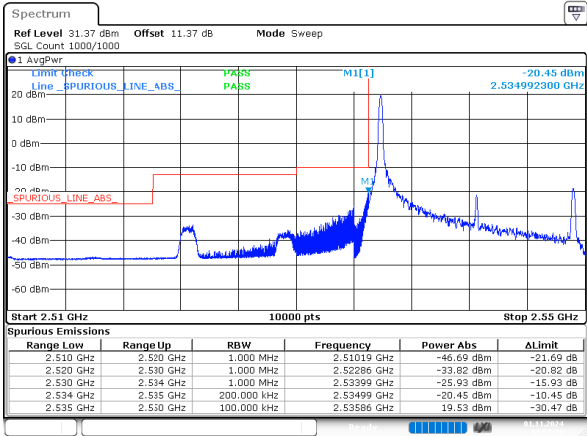
2_15MHz_Low_16QAM_1@0
