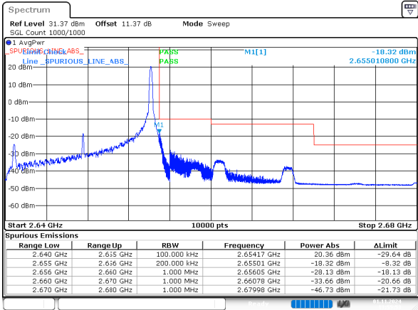
2_15MHz_High_QPSK_1@74
