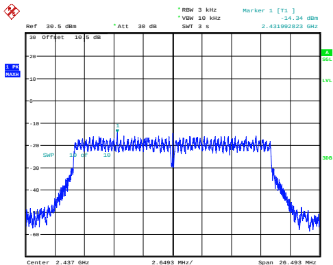
n20_2437MHz_Chain 0 -14.34dBm/3kHz
