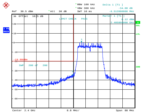
n20_2412MHz_Chain 0 34.00dB
