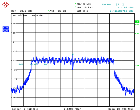
n20_2412MHz_Chain 0 -14.69dBm/3kHz
