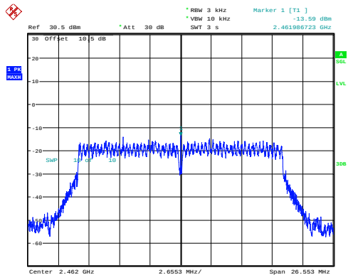
n20_2462MHz_Chain 0 -13.59dBm/3kHz
