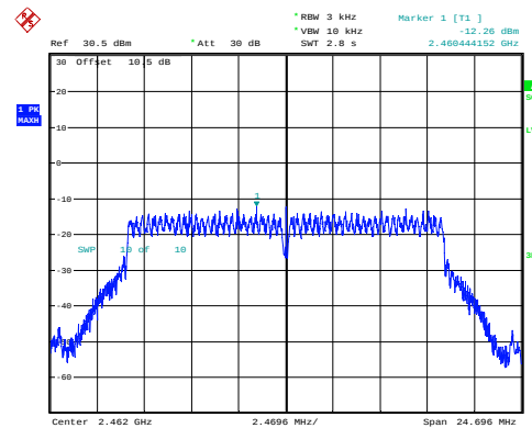
g_2462MHz_Chain 0 -12.26dBm/3kHz
