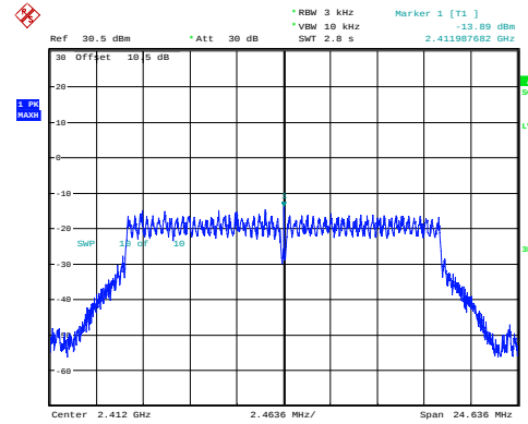
g_2412MHz_Chain 0 -13.89dBm/3kHz
