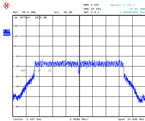
g_2437MHz_Chain 0 -12.51dBm/3kHz
