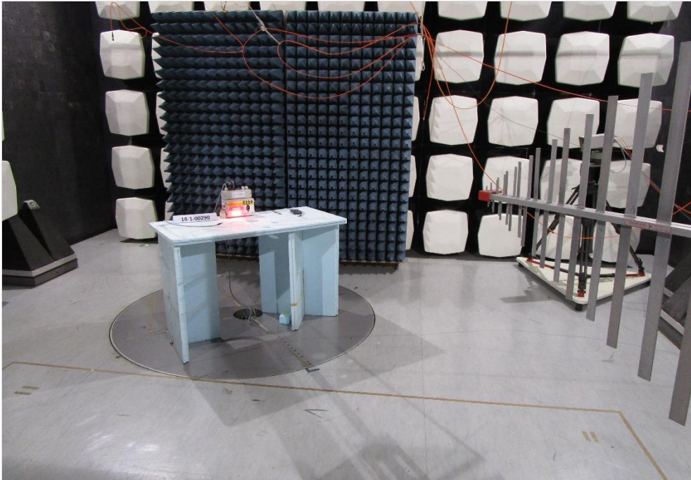
Photograph 1: EUT Test Setup in the anechoic chamber, Radiated interference field strength below 1GHz
