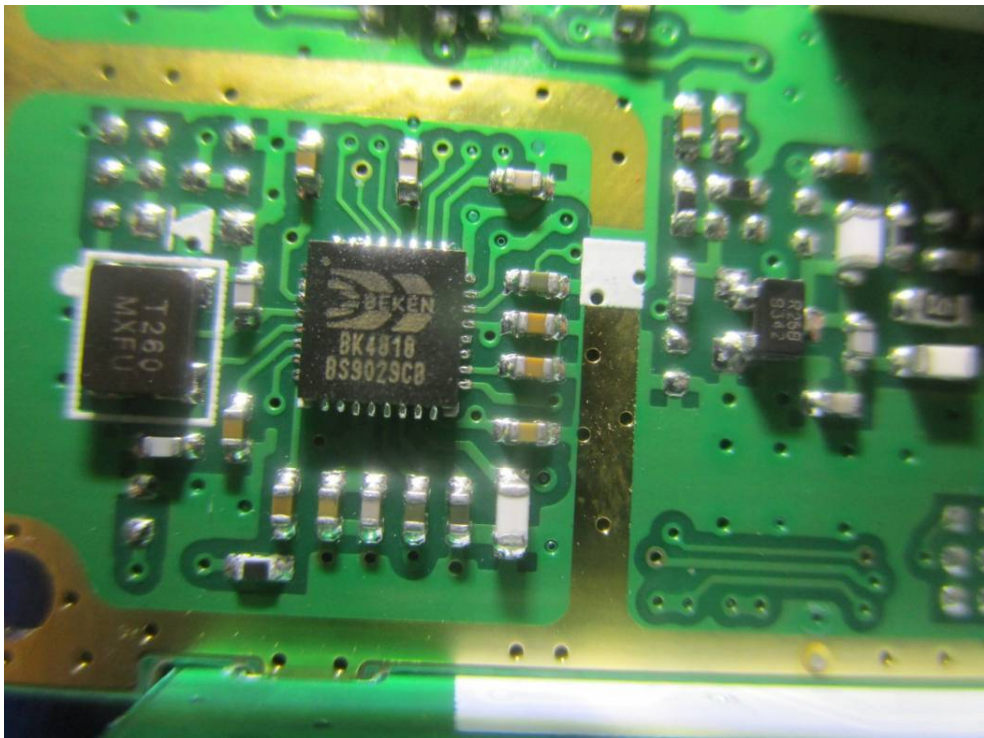
Chip View
