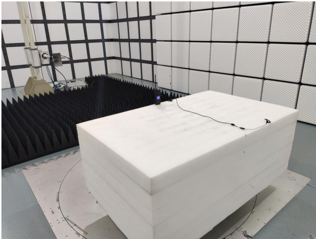
Radiated Emissions Test View (Above 1GHz)-Test Mode 2~7
