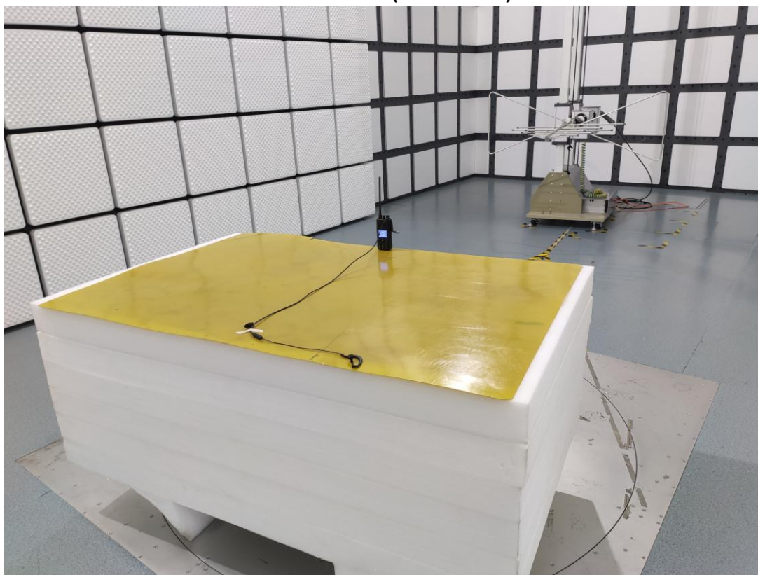
Radiated Emissions Test View (Below 1GHz)-Test Mode 1&8
