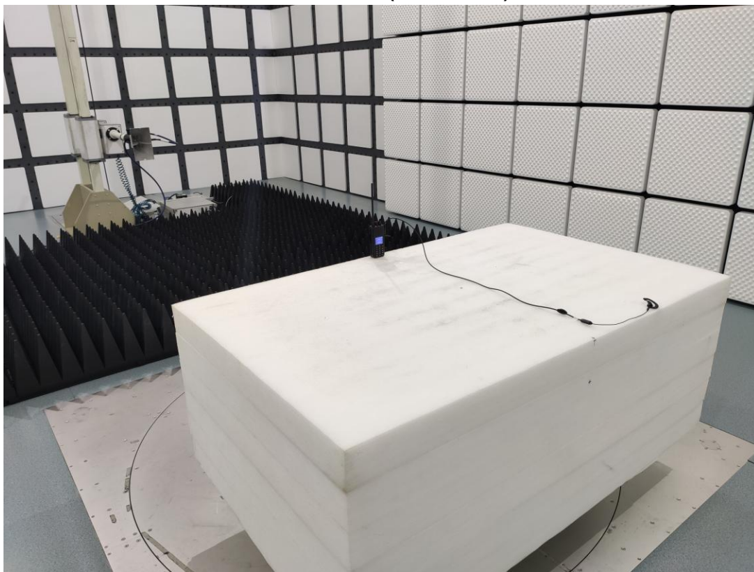
Radiated Emissions Test View (Above 1GHz)-Test Mode 1&8
