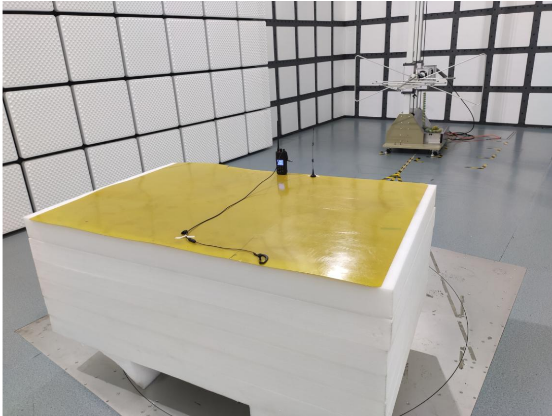
Radiated Emissions Test View (Below 1GHz)-Test Mode 2~7
