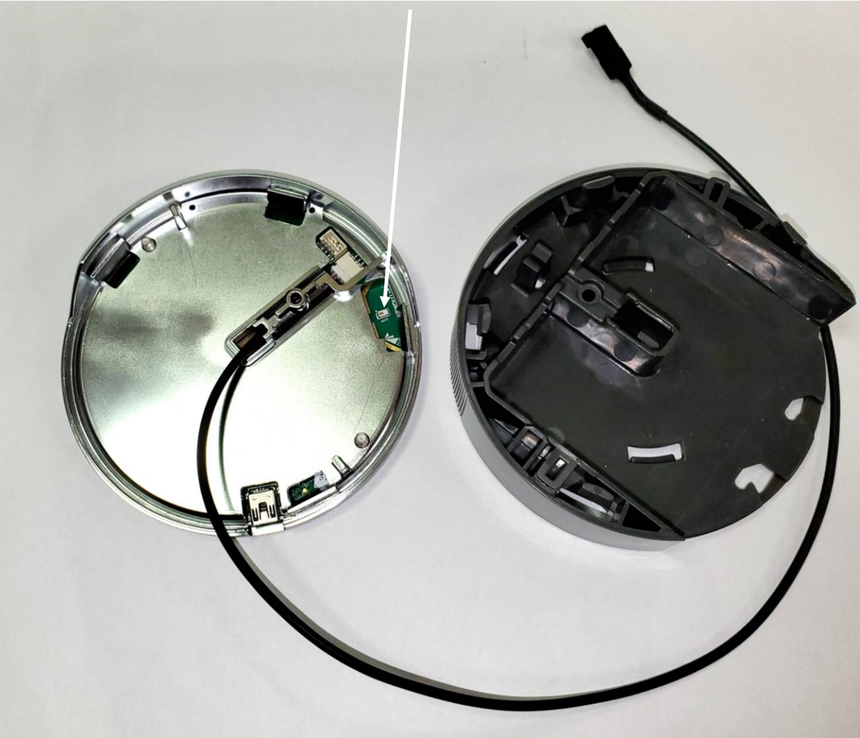
Chip Antenna
