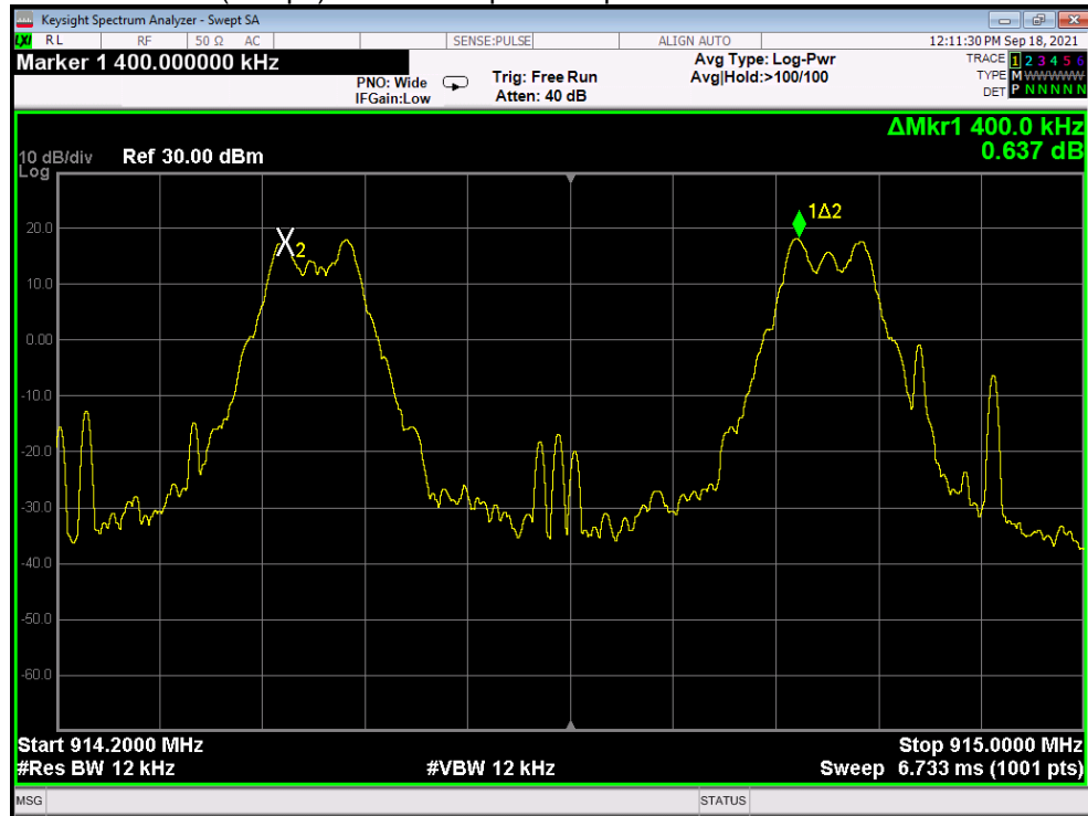
(1Mbps) Channel Separation plot on channel 63-64
