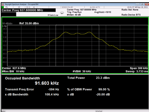
20dB Bandwidth plot on channel 64 (1Mbps)
