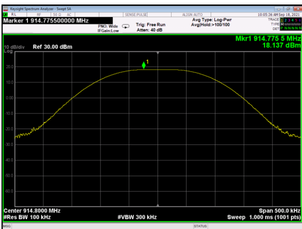
Peak output Power plot on channel 32 (1Mbps)
