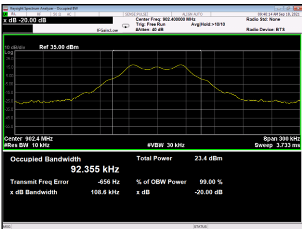
20dB Bandwidth plot on channel 32 (1Mbps)
