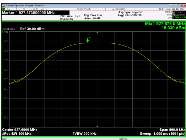
Peak output Power plot on channel 64(1Mbps)
