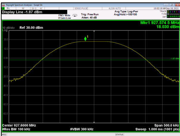
GFSK on channel 64
