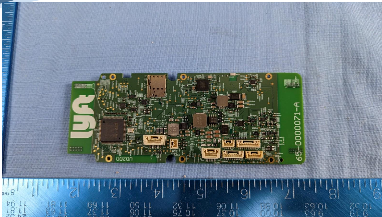
Internal PCB Top
