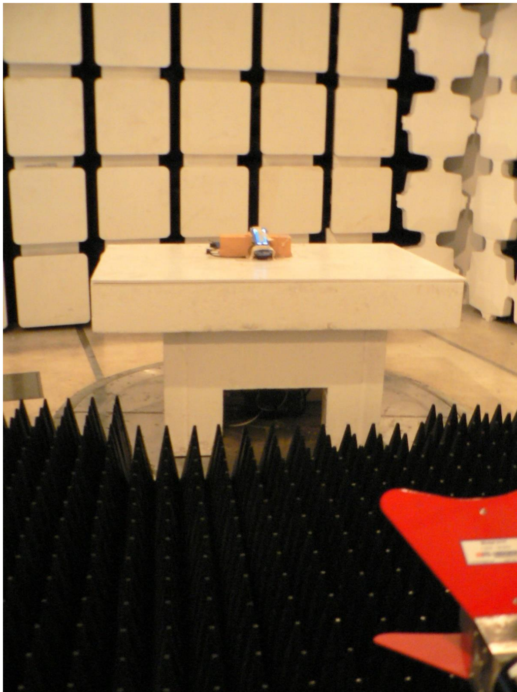
LYFT08 Digital Emissions 1-18GHz
