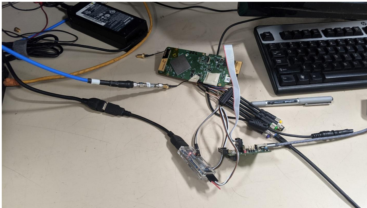
Conducted NFC Test Setup
