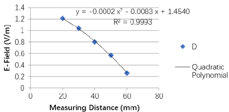
Position D E-Field
