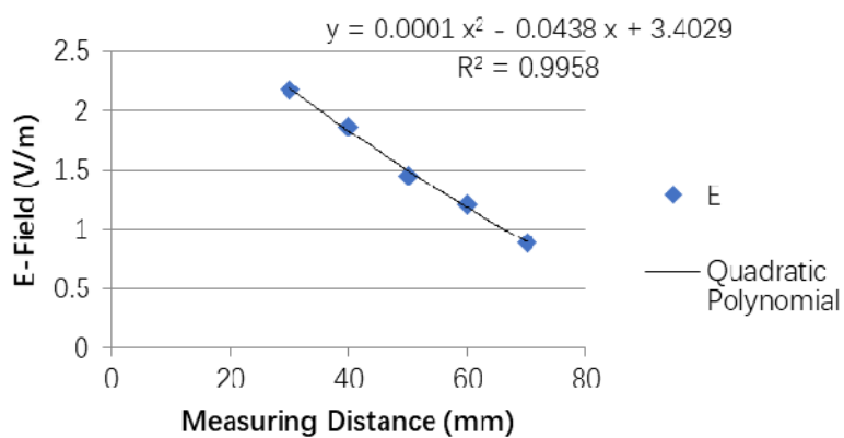
Position E E-Field
