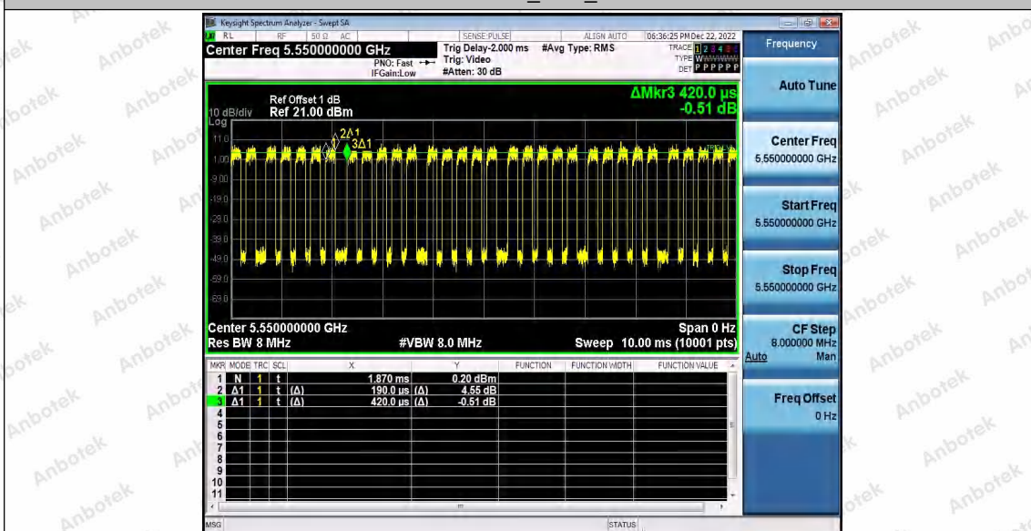
11AC40SISO_Ant1_5550
