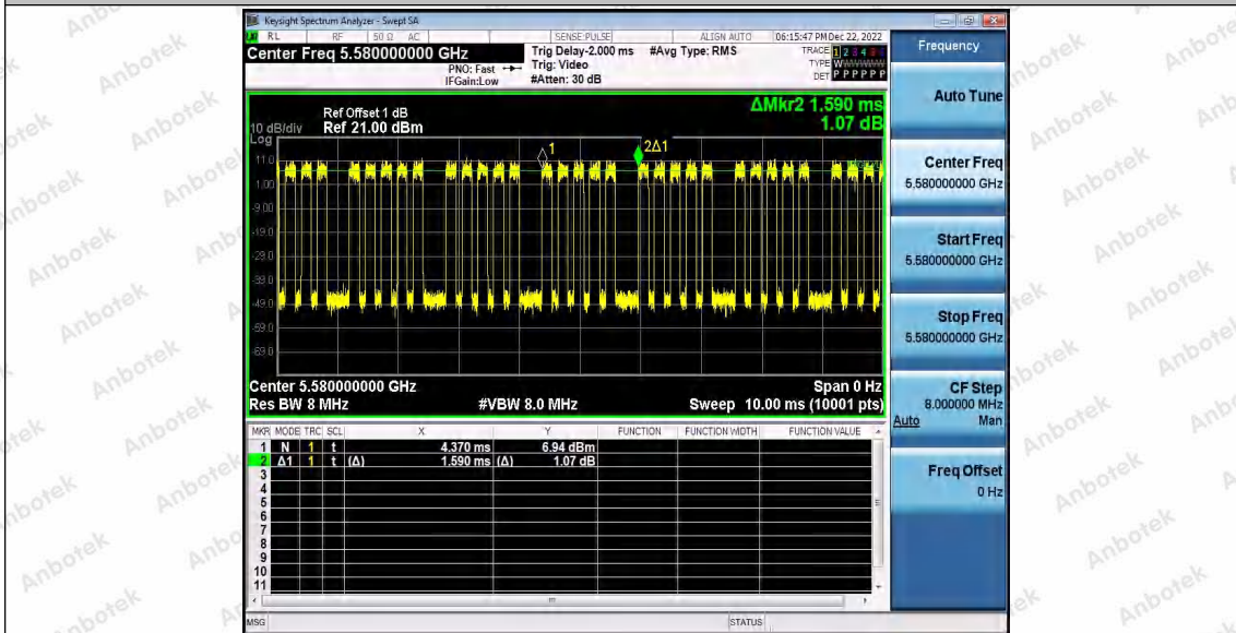
11AC20SISO_Ant2_5580
