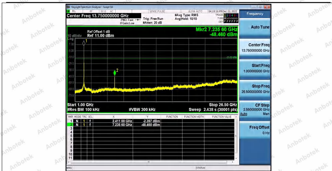
11G_Ant2_2412_0~Reference
