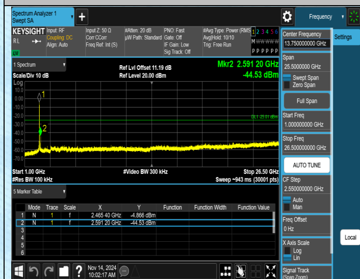
11N20SISO-Ant1-2462-1000~26500-PASS
