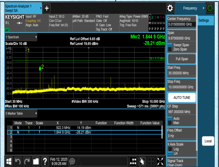
TX-Ant1-922.5-30~10000-PASS
