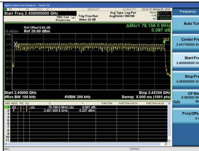
8DPSK Modulation
