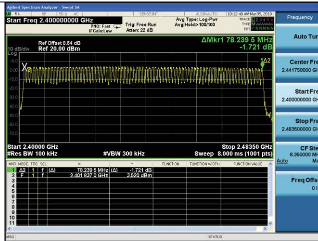
GFSK Modulation
