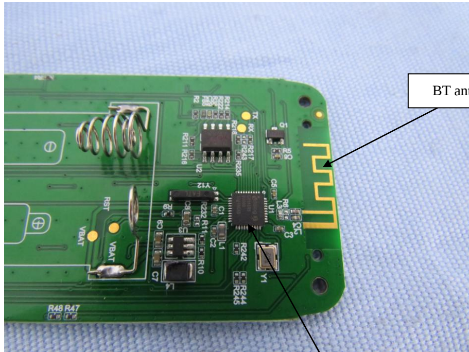
BT chip
