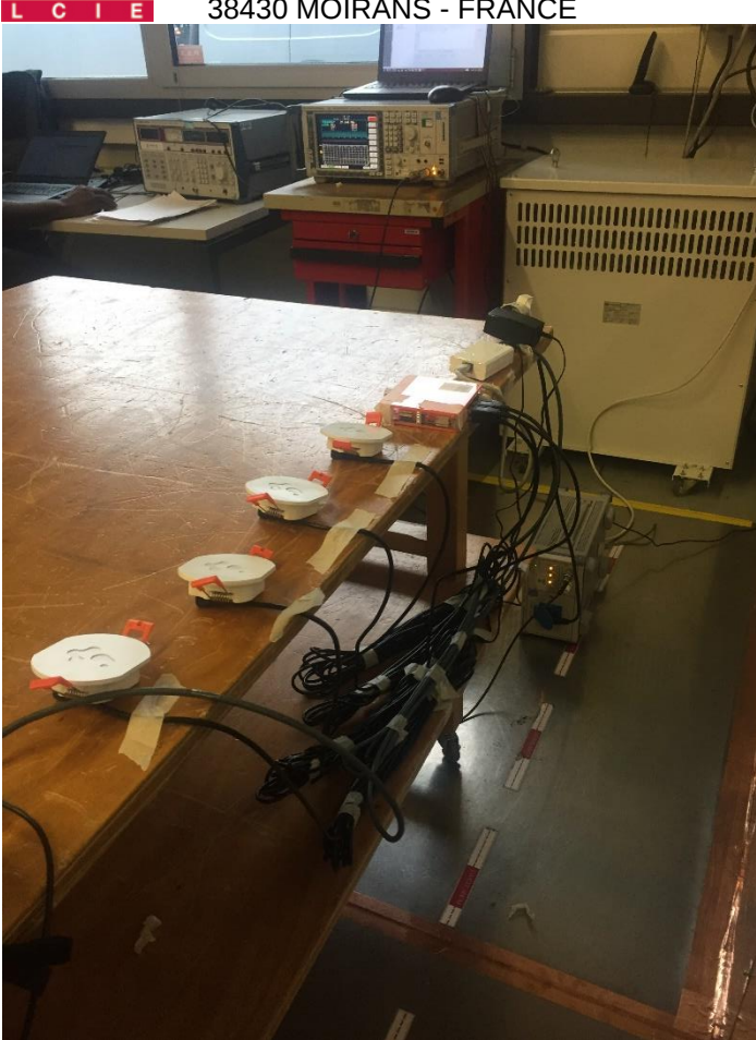
Test setup
