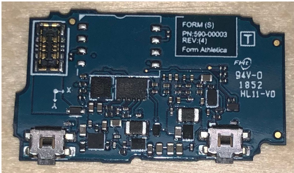
PCBA only (bottom side):
