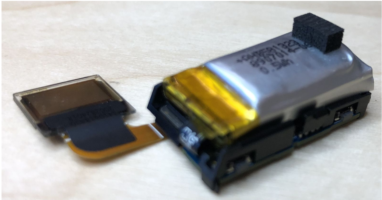
Electronics removed from enclosure (perspective 1):
