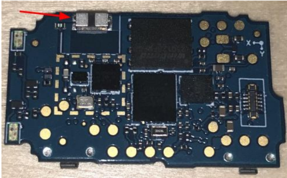
PCBA only (top side, antenna indicated with red arrow):
