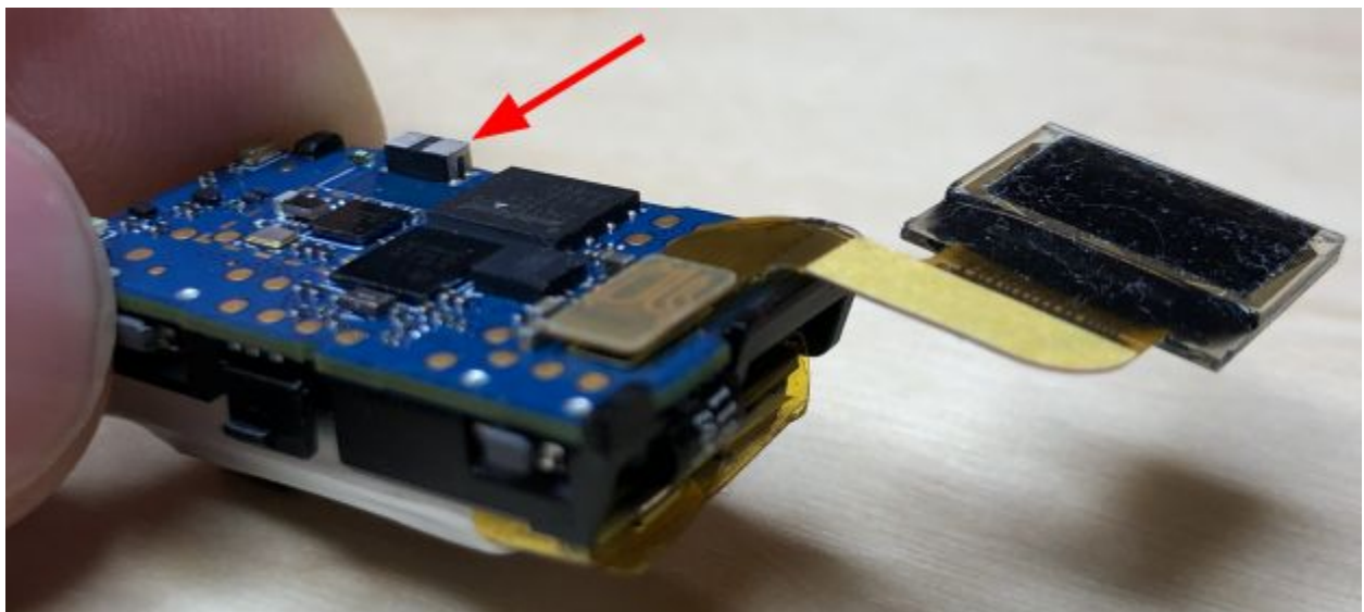
Electronics removed from enclosure (perspective 2, antenna indicated with red arrow):
