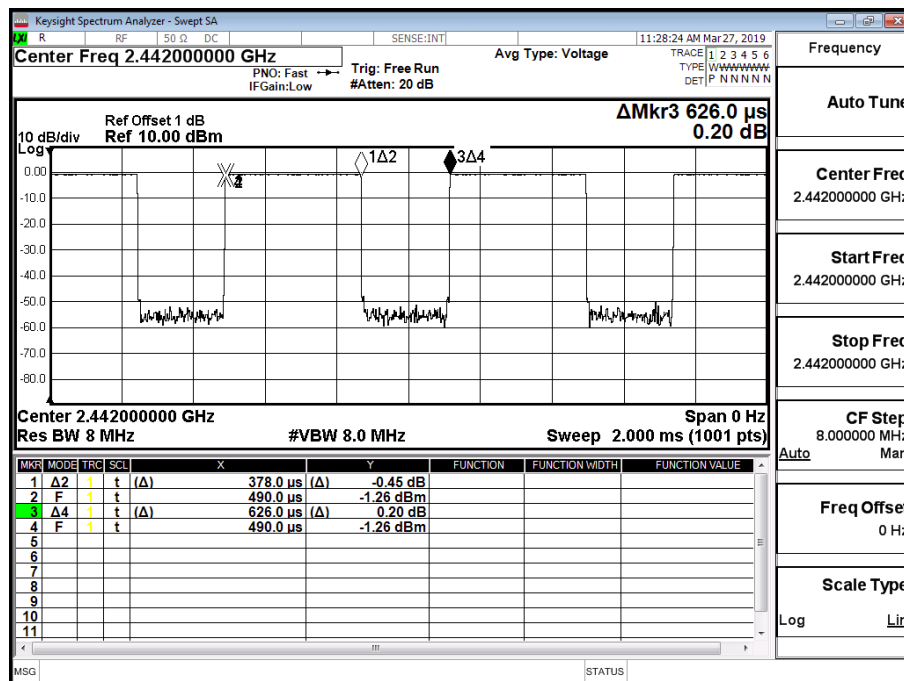
FCC_15_247_BT4Duty Cycle_BLE_1M_MidCH20-2442
