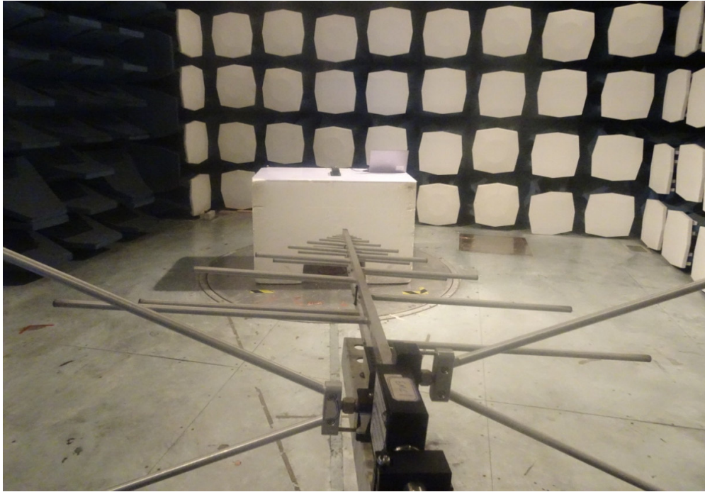
30MHz-1GHz
