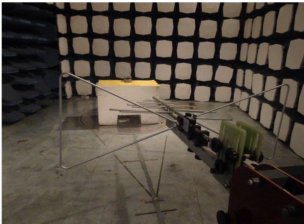
30MHz-1GHz
