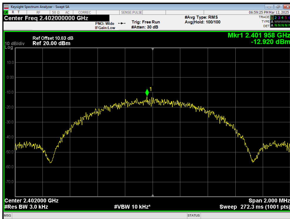
PSD NVNT Bluetooth LE 2402MHz
