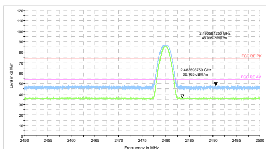
Bluetooth LE Channel 39 Peak+Average
