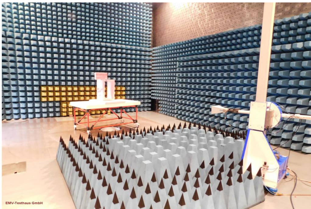
Picture 6: SAC, radiated emission 1 GHz – 10 GHz (rear view)
