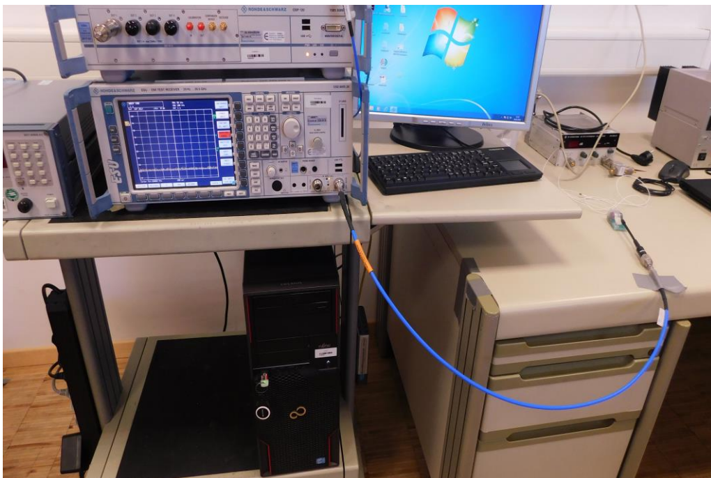
Picture 10: Relative measurements of duty cycle, signal deactivation and 20 dB bandwidth
