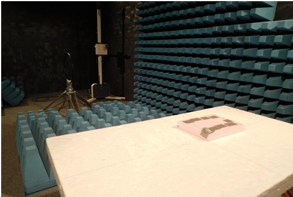
Picture 1: CDC, test setup radiated emission test 9 kHz -30 MHz (side view)
