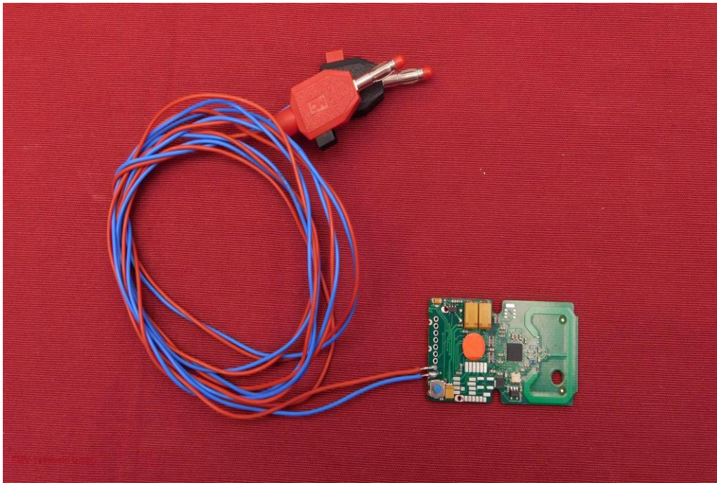
Picture 9: Transmitter without cover and power supply cables - top side
