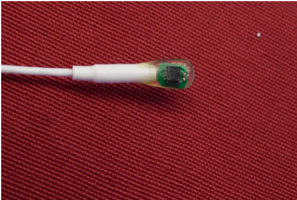
Picture 5: Sensor - top side
