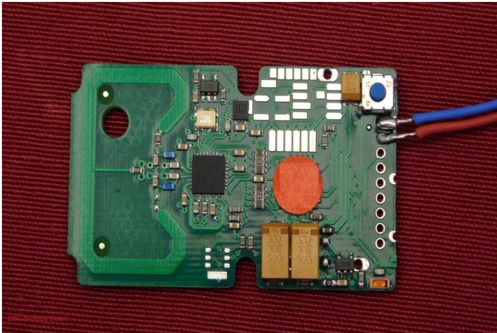
Picture 7: Transmitter without cover - top side
