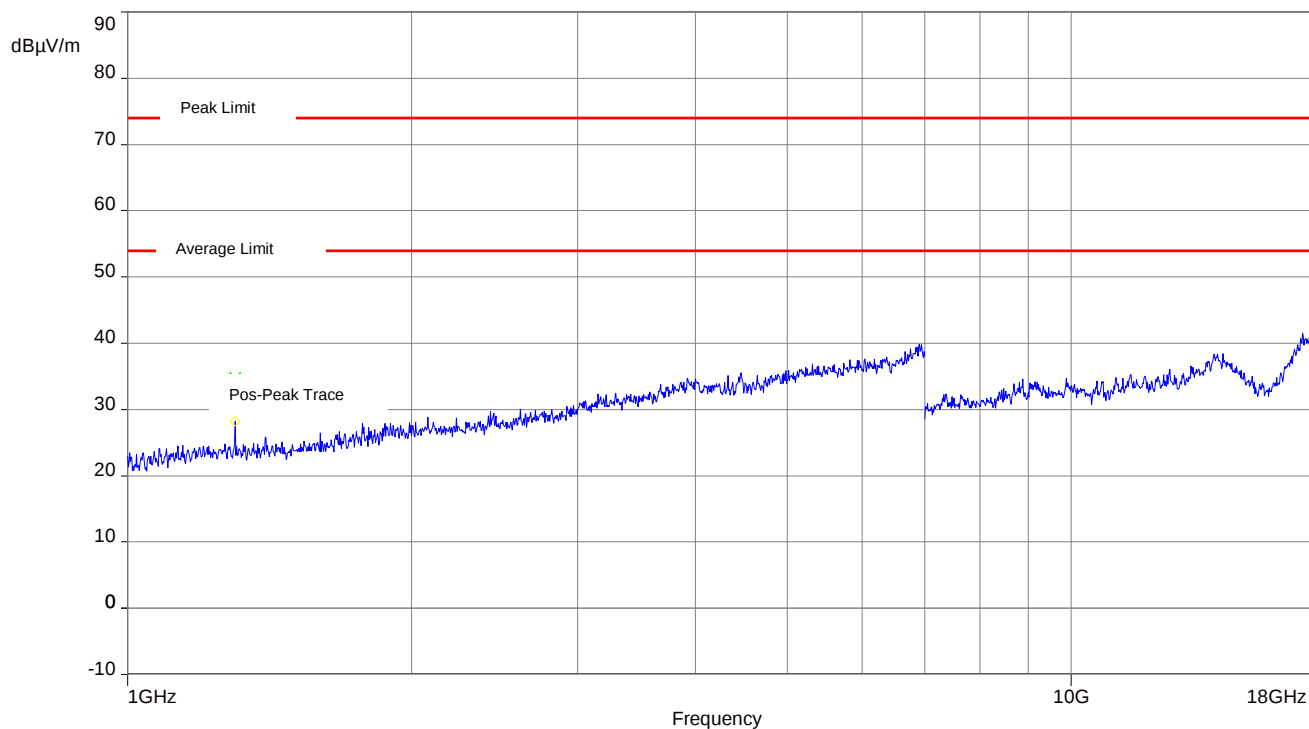
Plot 24: 1 GHz – 18 GHz, vertical / horizontal polarization, Mode 6
