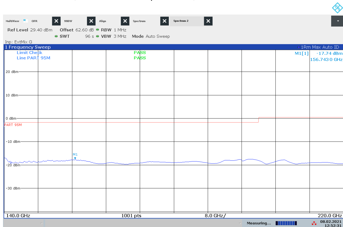
Plot 45: 140 GHz – 220 GHz, vertical / horizontal polarization, Mode 6
