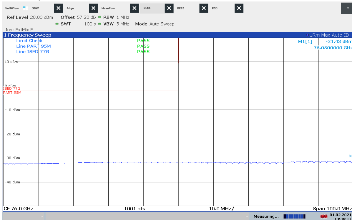
Plot 14: Mode 6, BEC
