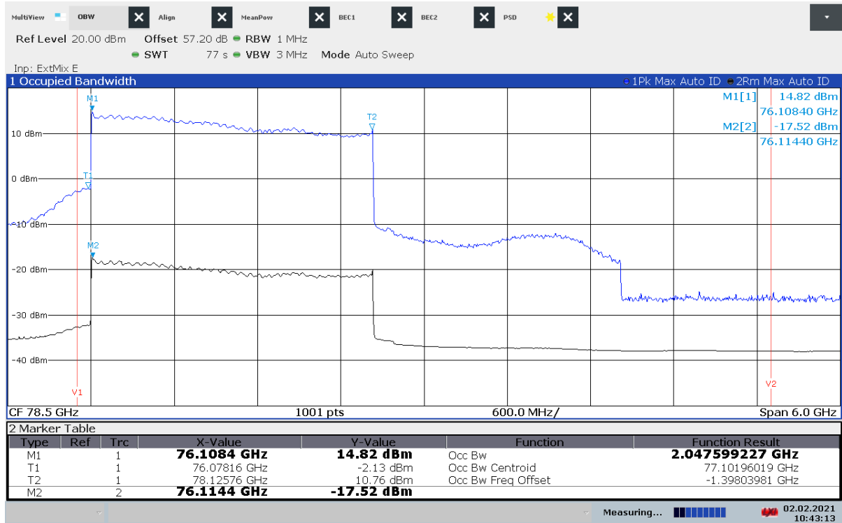
Plot 62: OBW, +20 °C / V_{nom} , Mode 5
