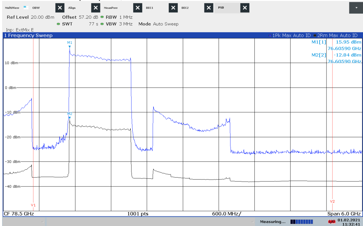
Plot 1: Mode 3 – Radiated peak power, PSD
