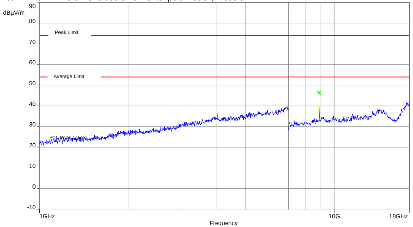
Plot 22: 1 GHz – 18 GHz, vertical / horizontal polarization, Mode 3
