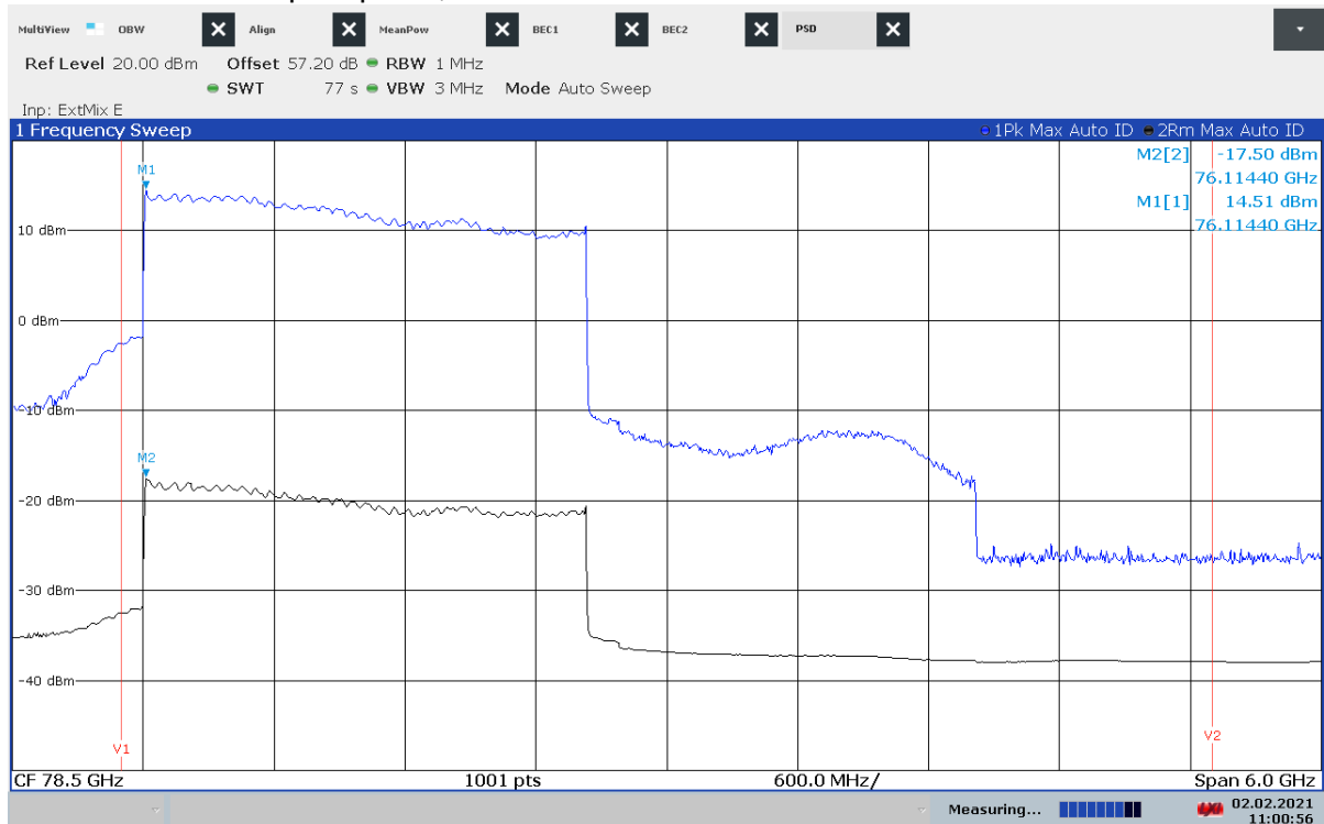
Plot 2: Mode 5 – Radiated peak power, PSD
