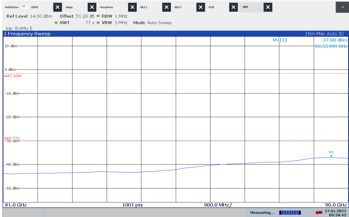
Plot 37: 81 GHz – 90 GHz, vertical / horizontal polarization, Mode 3
