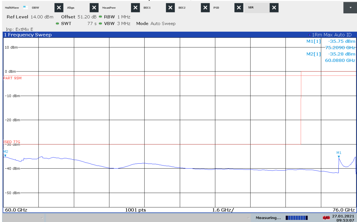
Plot 34: 60 GHz – 76 GHz, vertical / horizontal polarization, Mode 3
