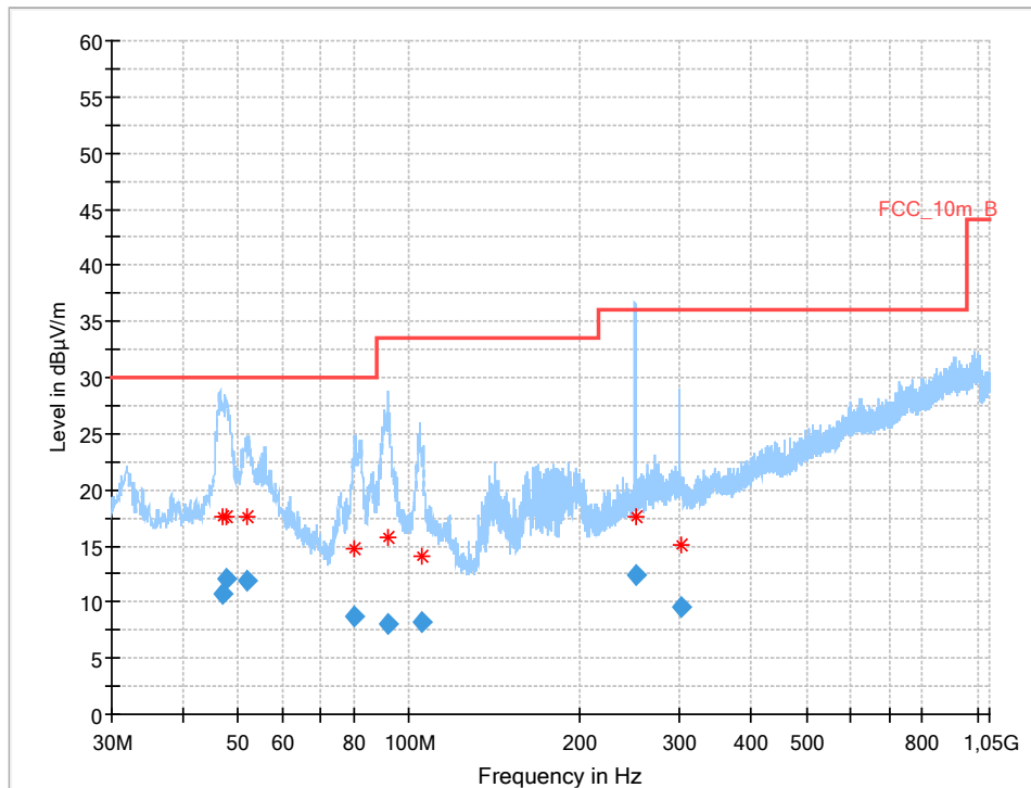
Plot 20: 30 MHz – 1 GHz, vertical / horizontal polarization, Mode 5
