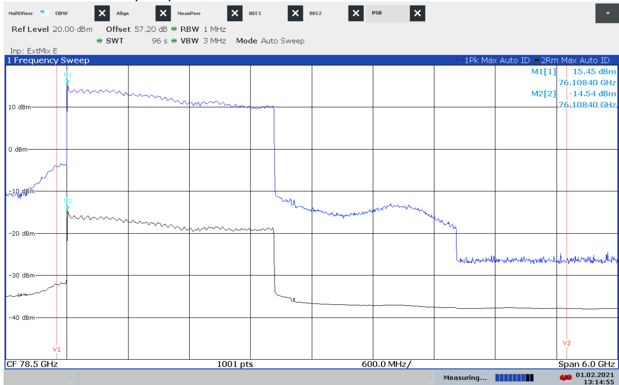
Plot 3: Mode 6 – Radiated peak power, PSD
