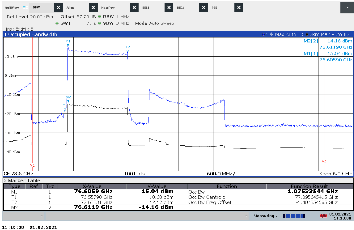
Plot 61: OBW, +20 °C / V_{nom} , Mode 3
