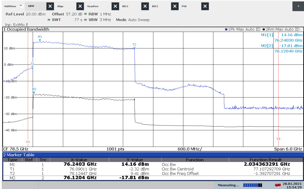
Plot 71: OBW, +50 °C / V_{nom} , Mode 5
