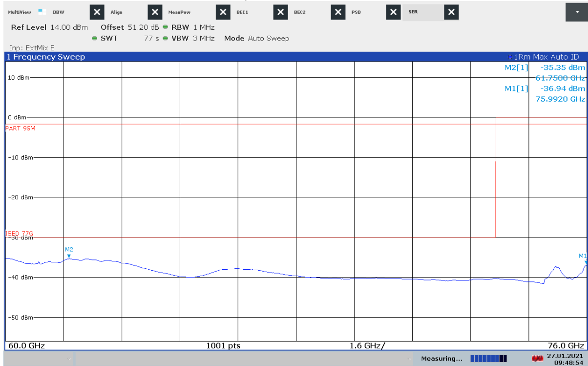
Plot 35: 60 GHz – 76 GHz, vertical / horizontal polarization, Mode 5
