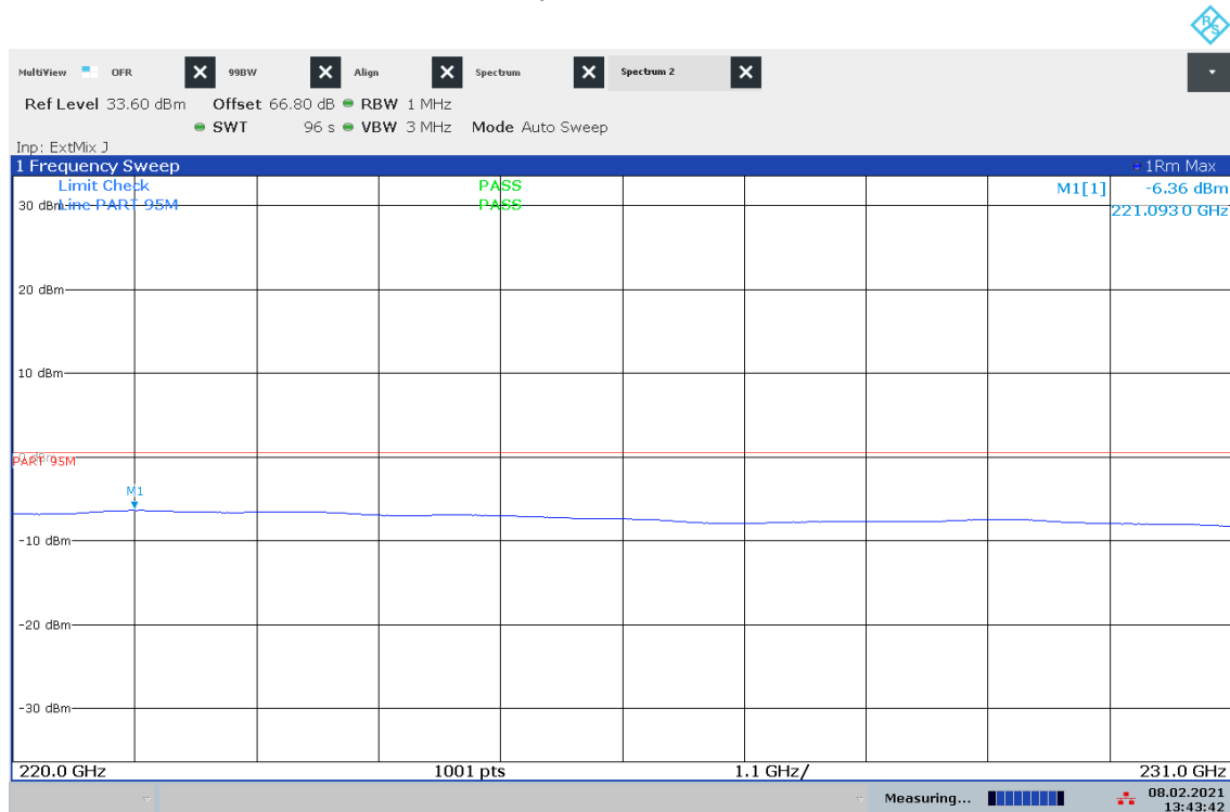
Plot 48: 220 GHz – 231 GHz, vertical / horizontal polarization, Mode 6
