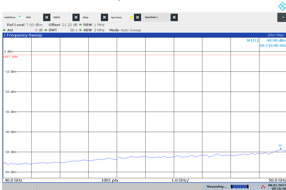
Plot 30: 40 GHz – 50 GHz, vertical / horizontal polarization, Mode 6
