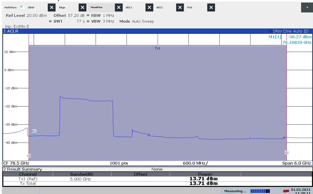
Plot 4: Mode 3 – Mean power
