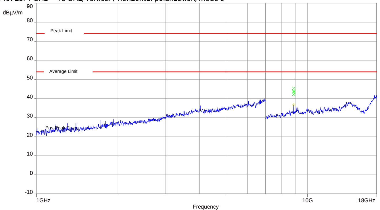
Plot 23: 1 GHz – 18 GHz, vertical / horizontal polarization, Mode 5
