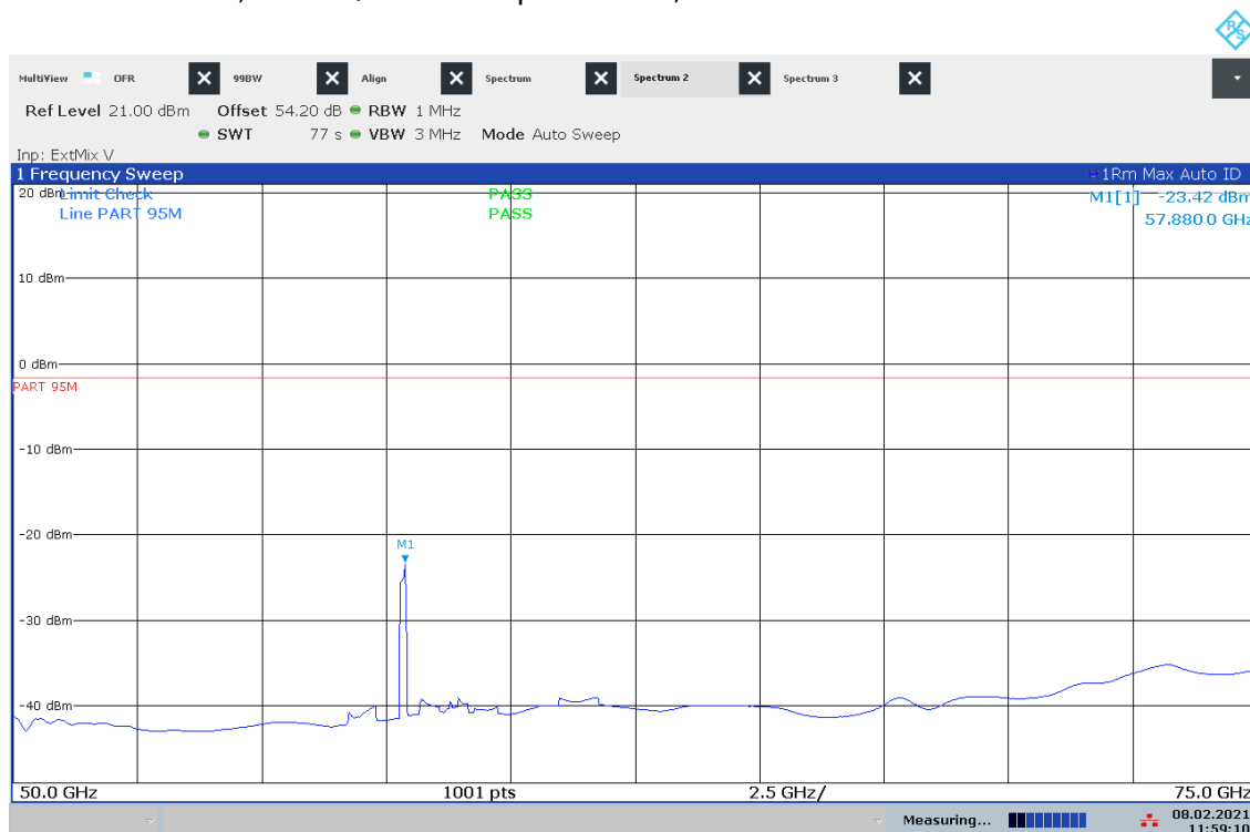
Plot 31: 50 GHz – 75 GHz, vertical / horizontal polarization, Mode 3
