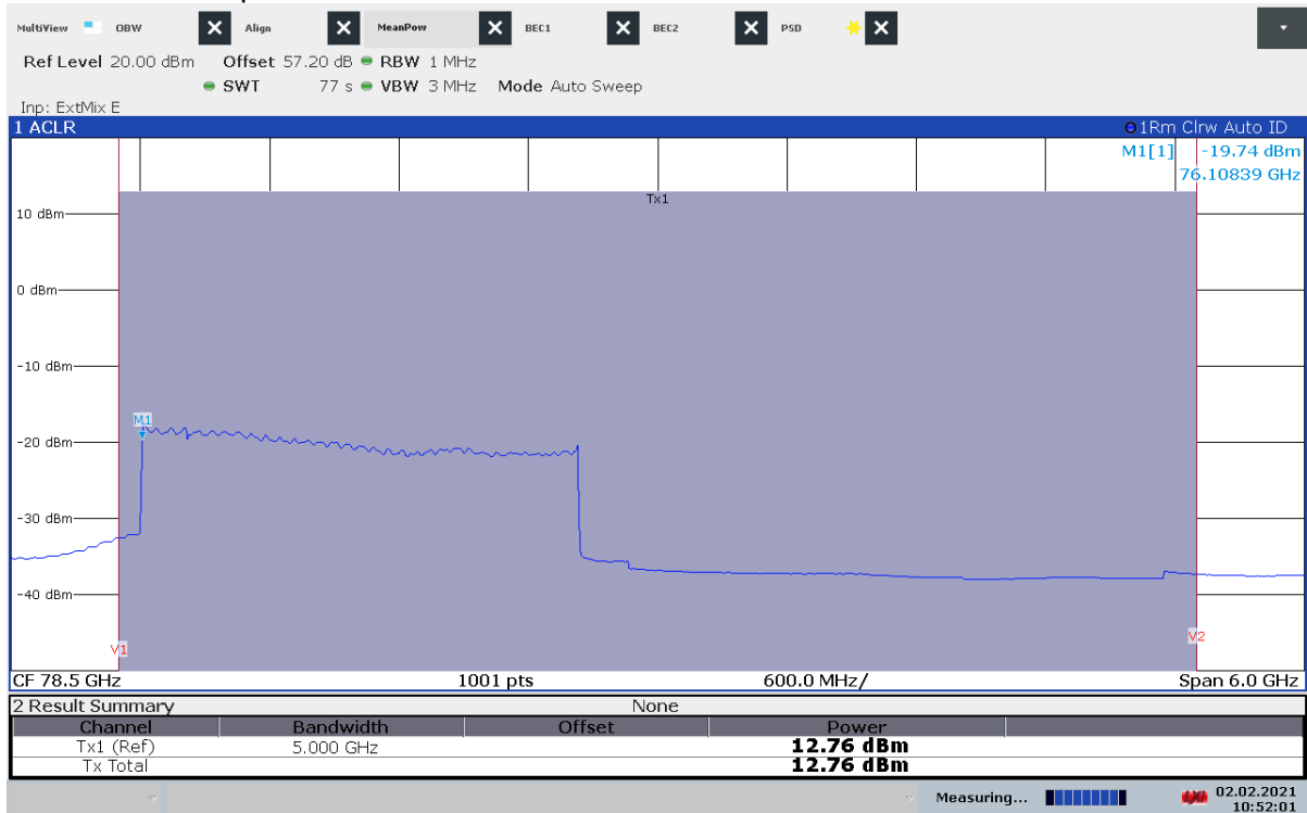
Plot 5: Mode 5 – Mean power
