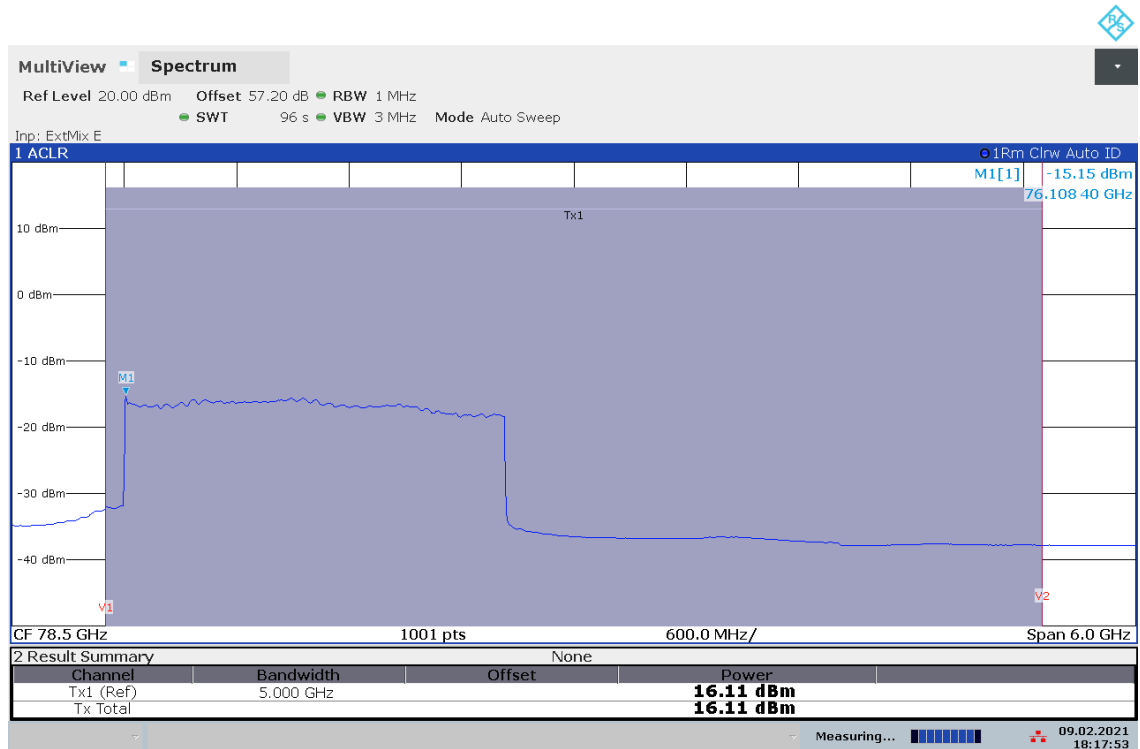
Plot 6: Mode 6 – Mean power
