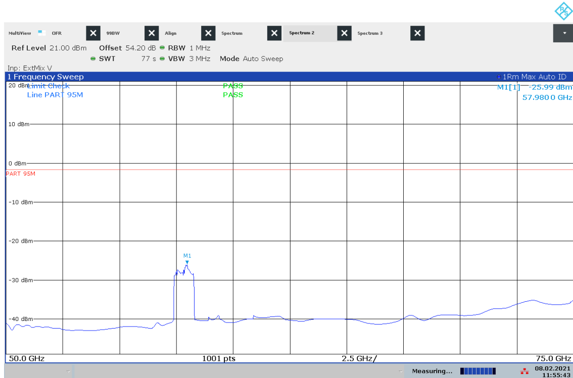
Plot 32: 50 GHz – 75 GHz, vertical / horizontal polarization, Mode 5
