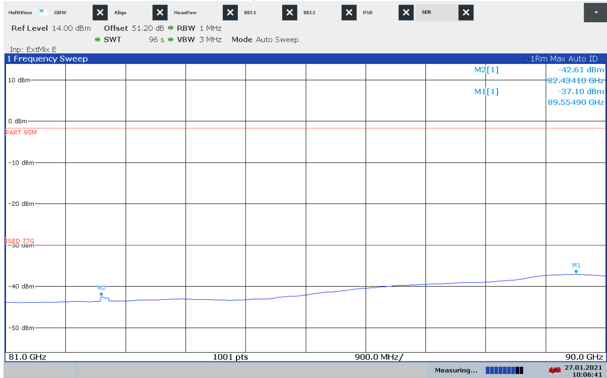
Plot 39: 81 GHz – 90 GHz, vertical / horizontal polarization, Mode 6
