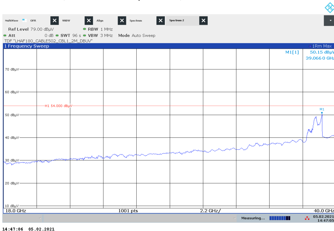
Plot 27: 18 GHz – 40 GHz, vertical / horizontal polarization, Mode 6
