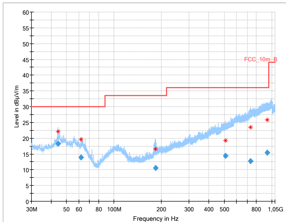
Plot 19: 30 MHz – 1 GHz, vertical / horizontal polarization, Mode 3
