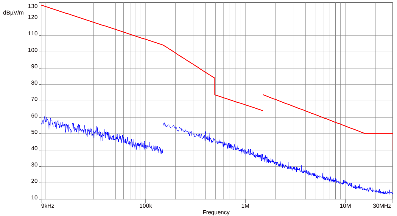
Plot 17: 9 kHz – 30 MHz, Magnetic antenna, Mode 5
