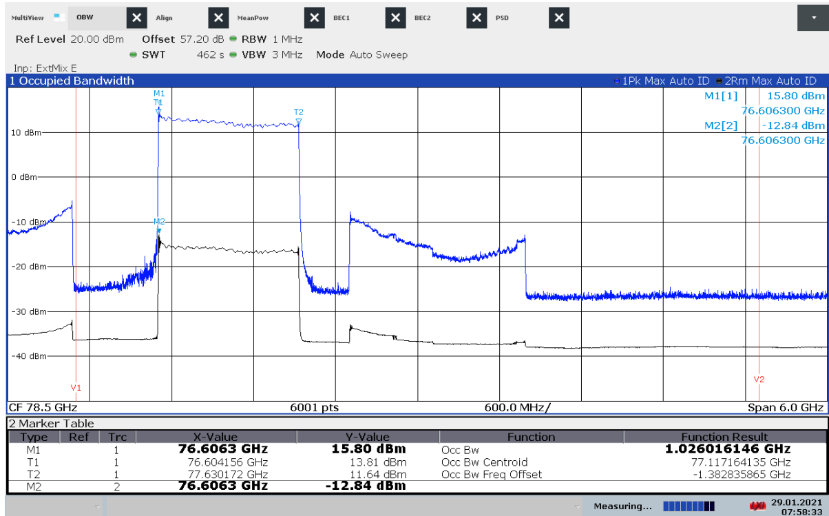
Plot 7: Mode 3 – OBW
