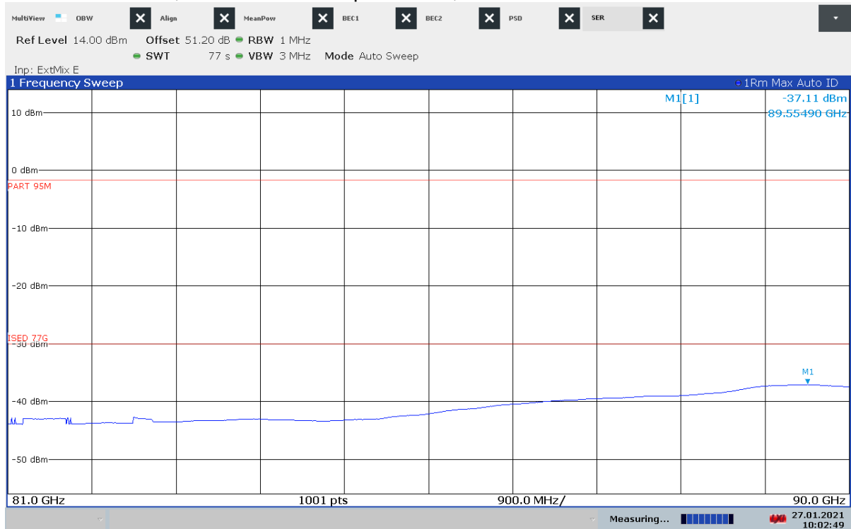
Plot 38: 81 GHz – 90 GHz, vertical / horizontal polarization, Mode 5
