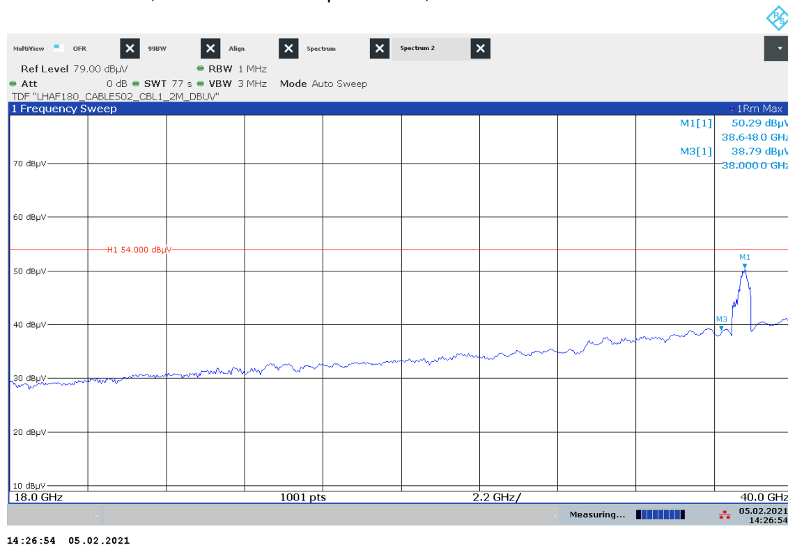
Plot 25: 18 GHz – 40 GHz, vertical / horizontal polarization, Mode 3
