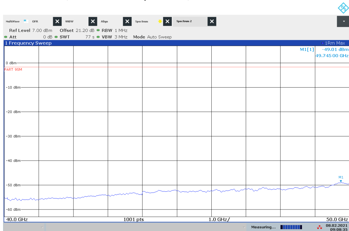
Plot 29: 40 GHz – 50 GHz, vertical / horizontal polarization, Mode 5
