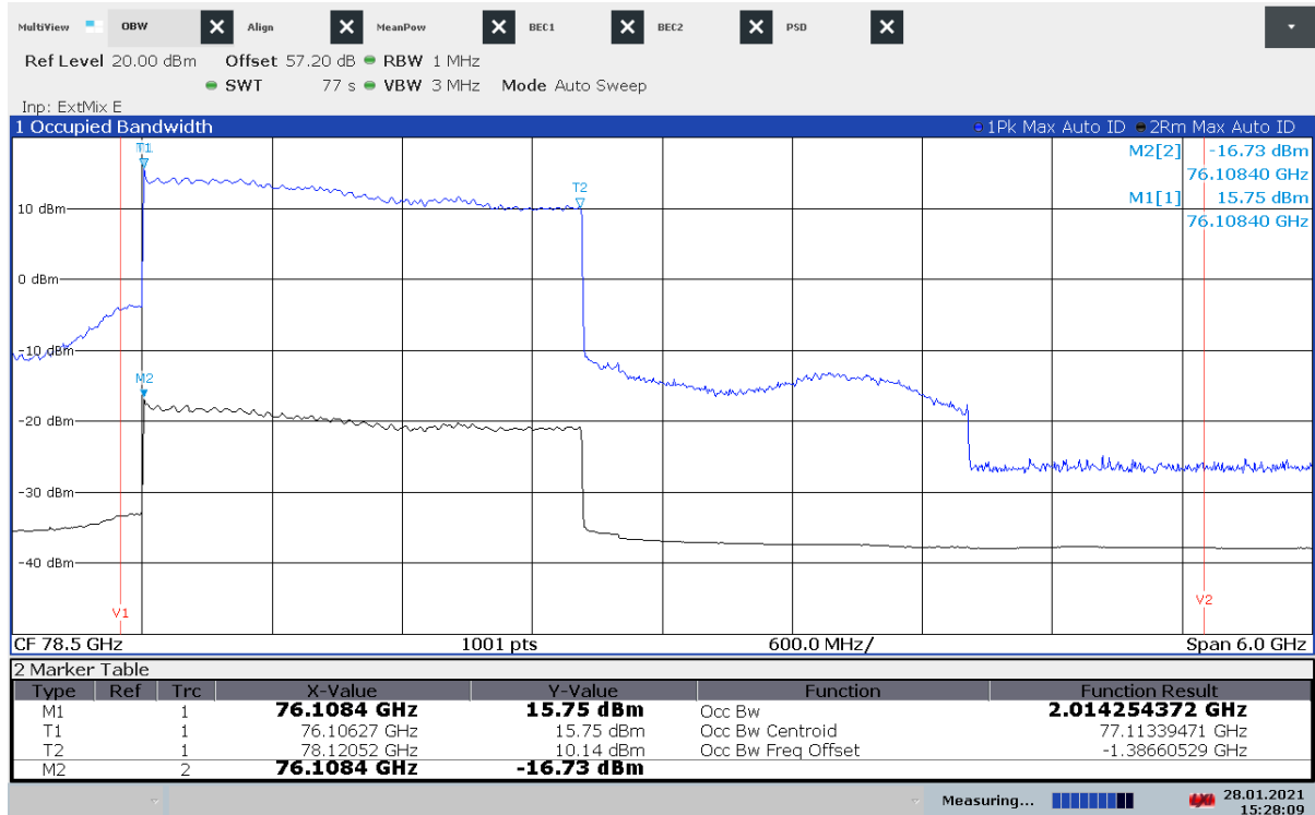
Plot 65: OBW, +30 °C / V_{nom} , Mode 5
