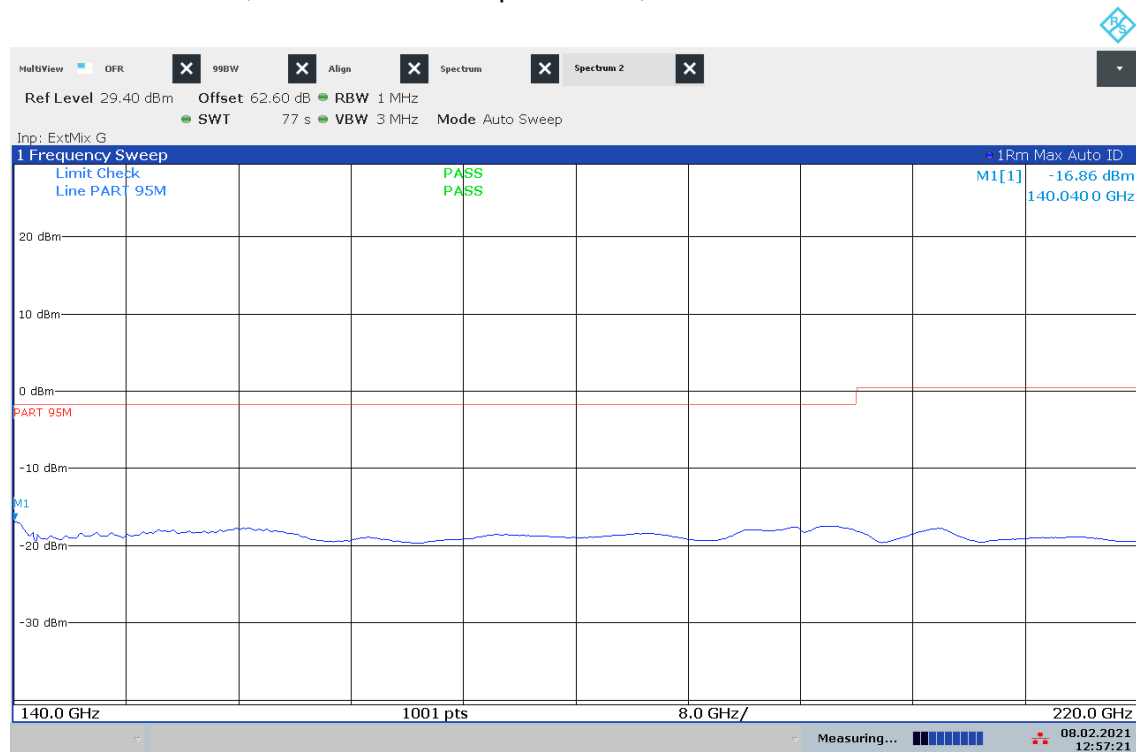
Plot 44: 140 GHz – 220 GHz, vertical / horizontal polarization, Mode 5
