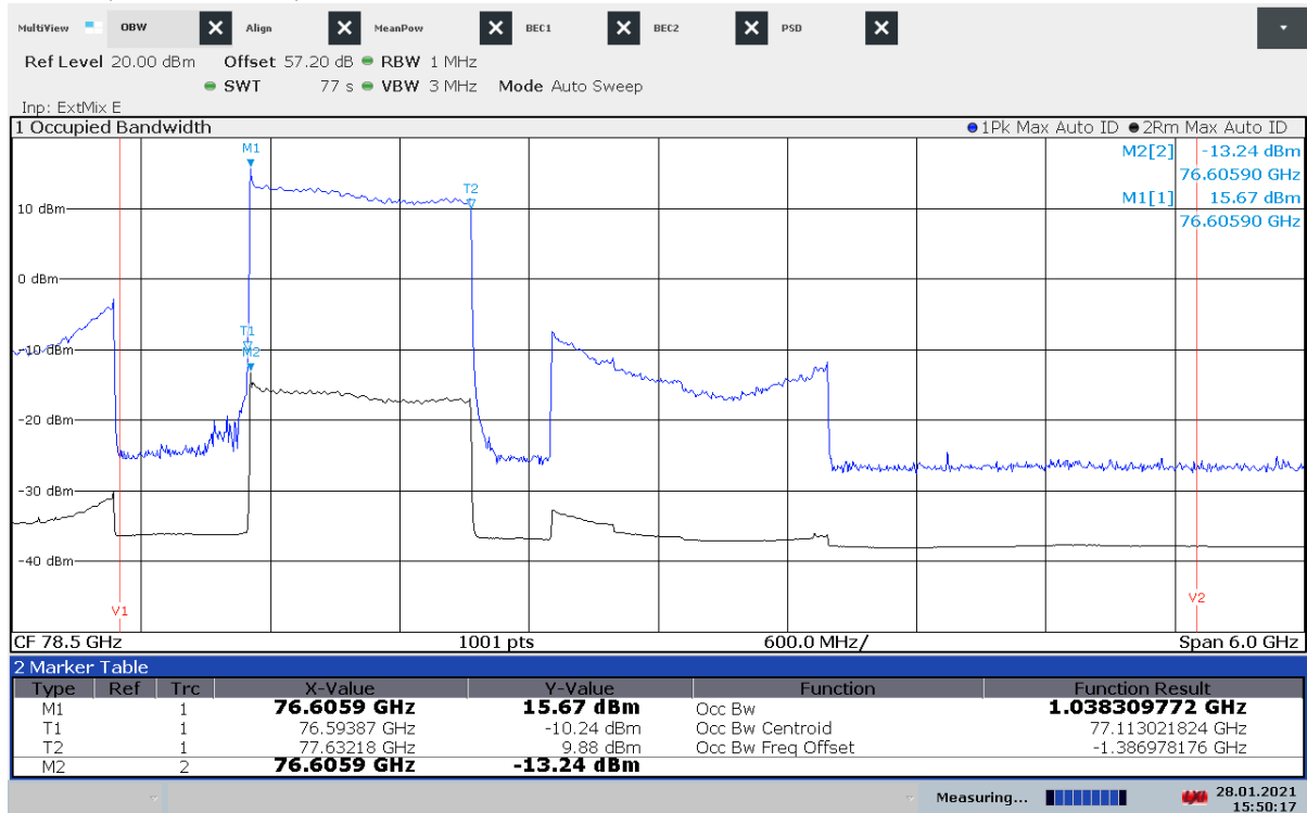
Plot 70: OBW, +50 °C / V_{nom} , Mode 3
