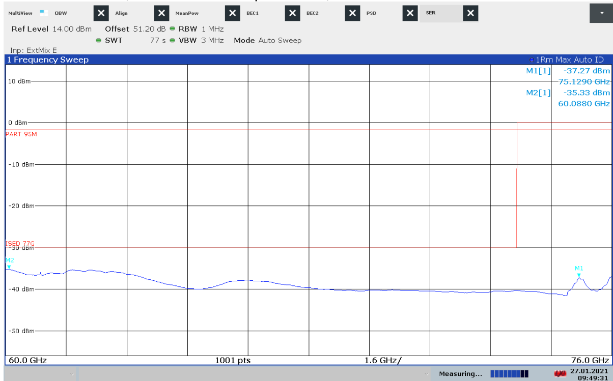
Plot 36: 60 GHz – 76 GHz, vertical / horizontal polarization, Mode 6
