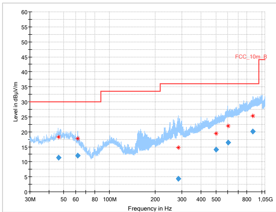
Plot 21: 30 MHz – 1 GHz, vertical / horizontal polarization, Mode 6
