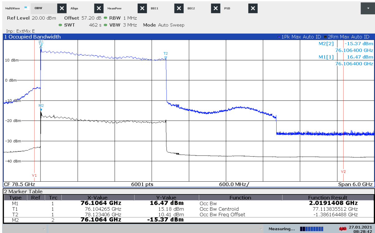
Plot 8: Mode 5 – OBW
