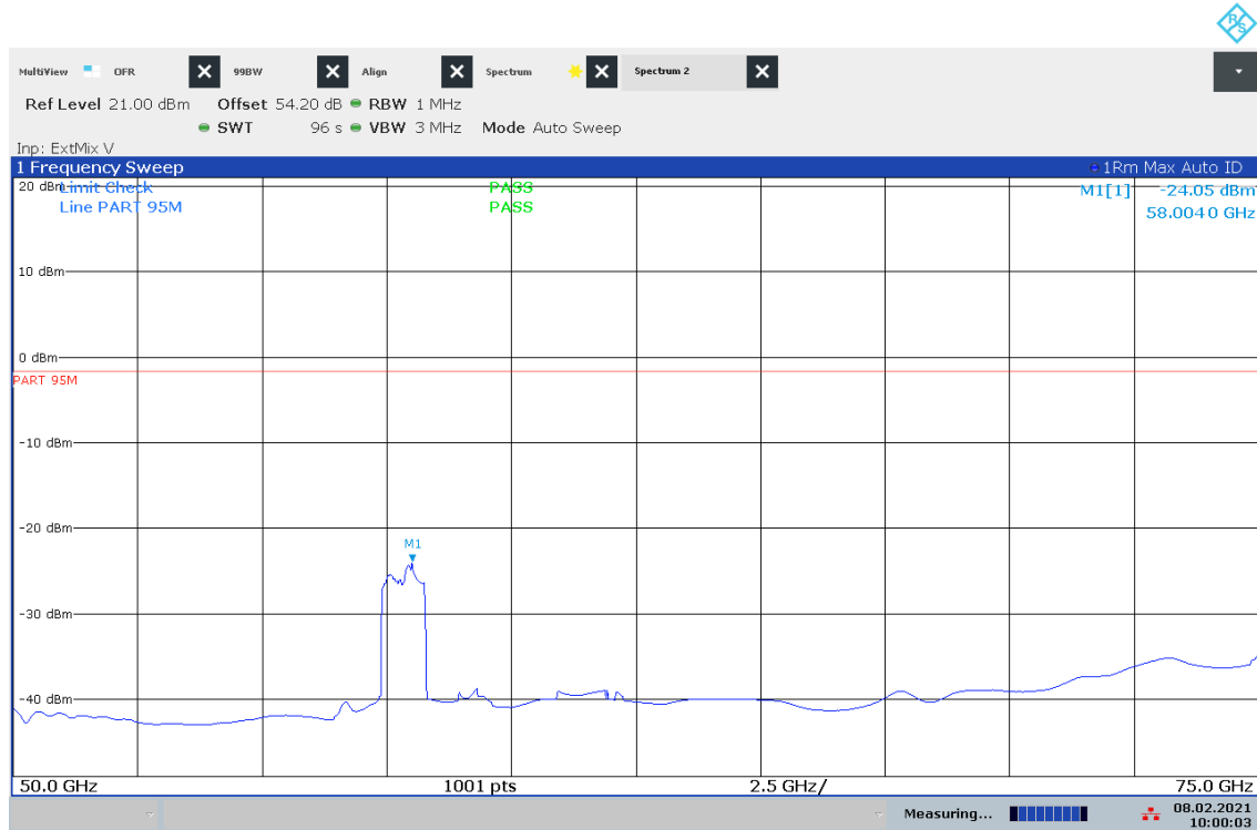
Plot 33: 50 GHz – 75 GHz, vertical / horizontal polarization, Mode 6
