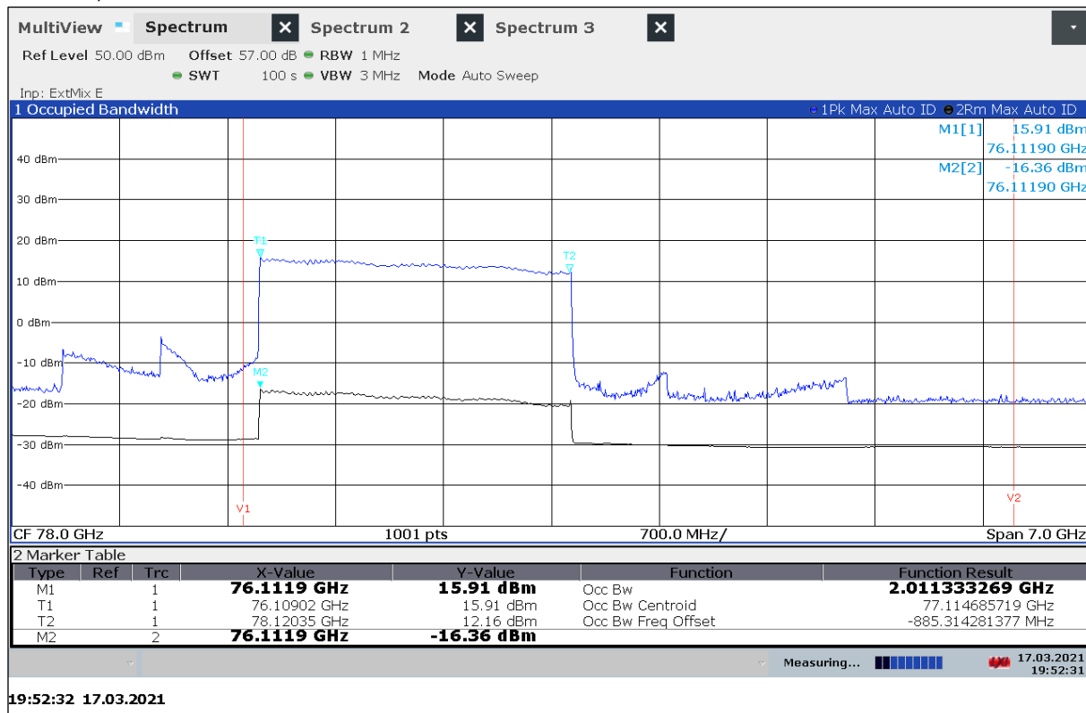
Plot 26: OBW, 10 °C / V_{nom}
