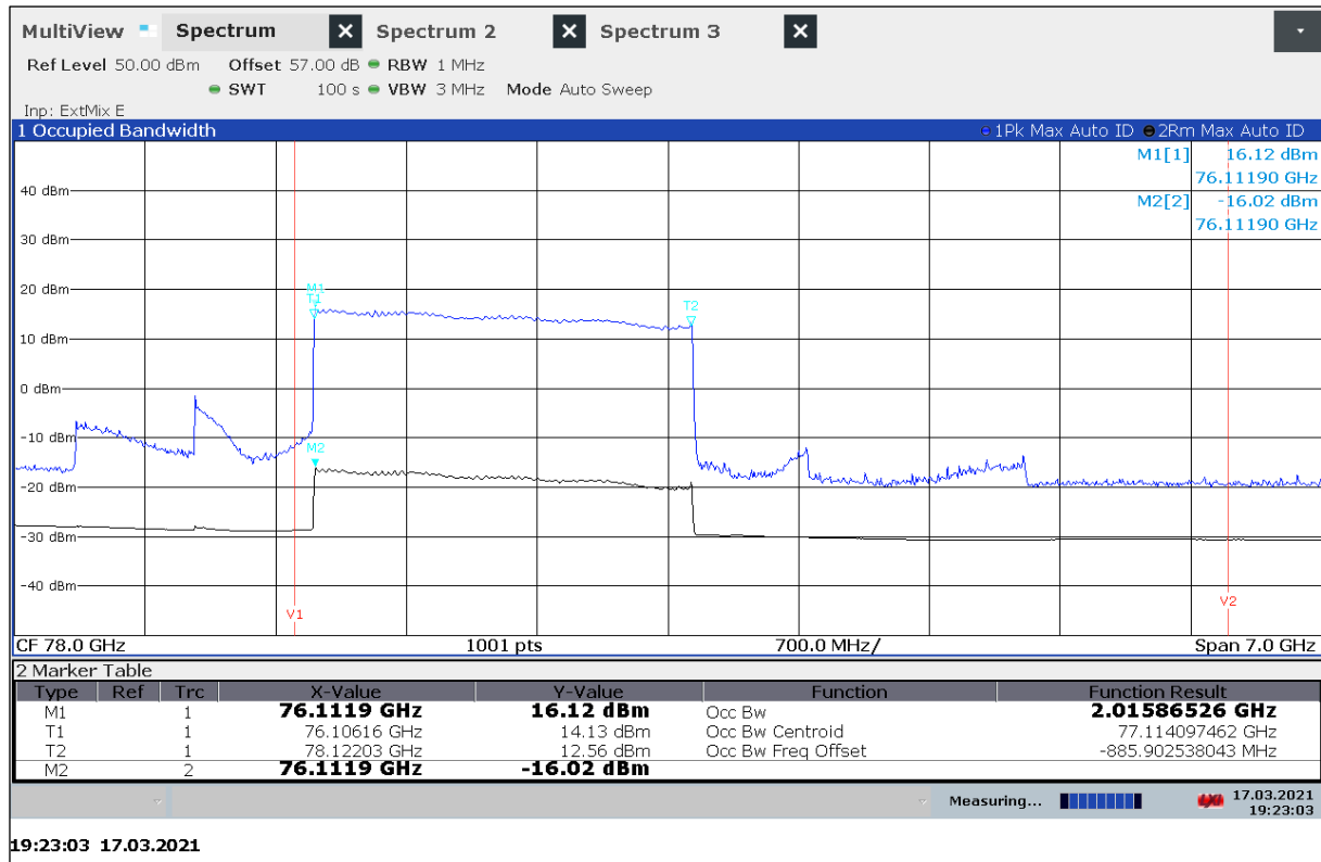
Plot 24: OBW, -10 °C / V_{nom}
