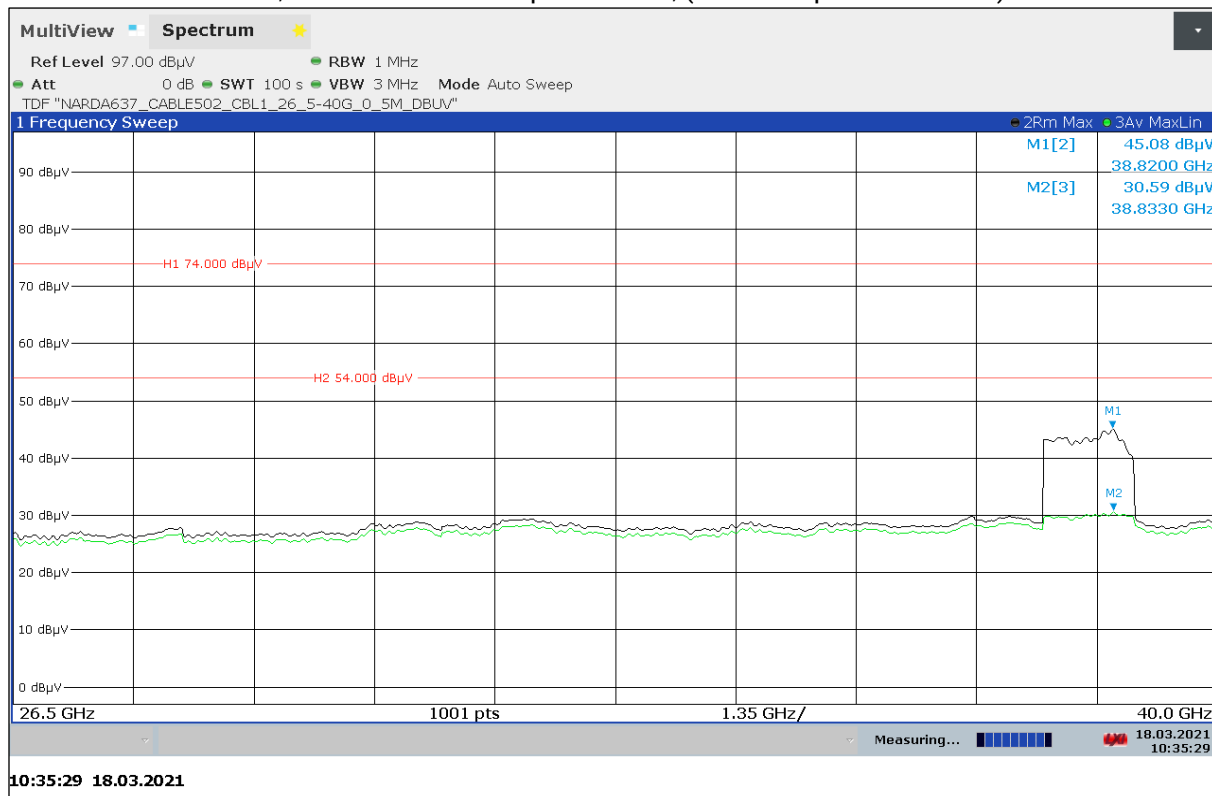
Plot 14: 26.5 GHz – 40 GHz, vertical / horizontal polarization, (Valid for specified Modes)
