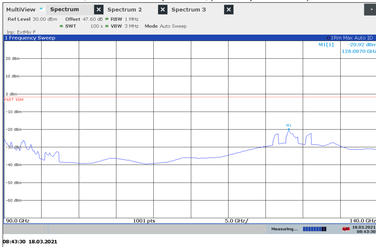
Plot 20: 90 GHz – 140 GHz, vertical / horizontal polarization, (Valid for specified Modes)
