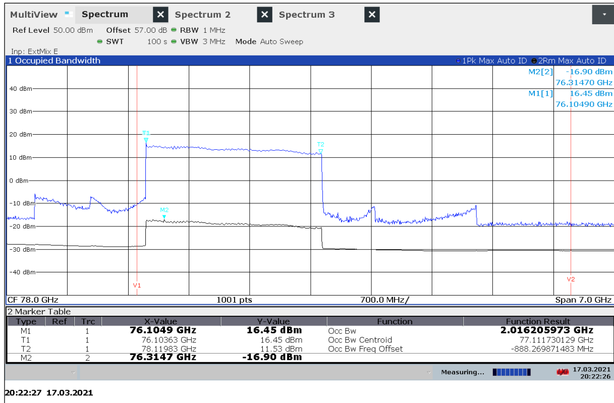
Plot 27: OBW, 20 °C / V_{\min-max}
