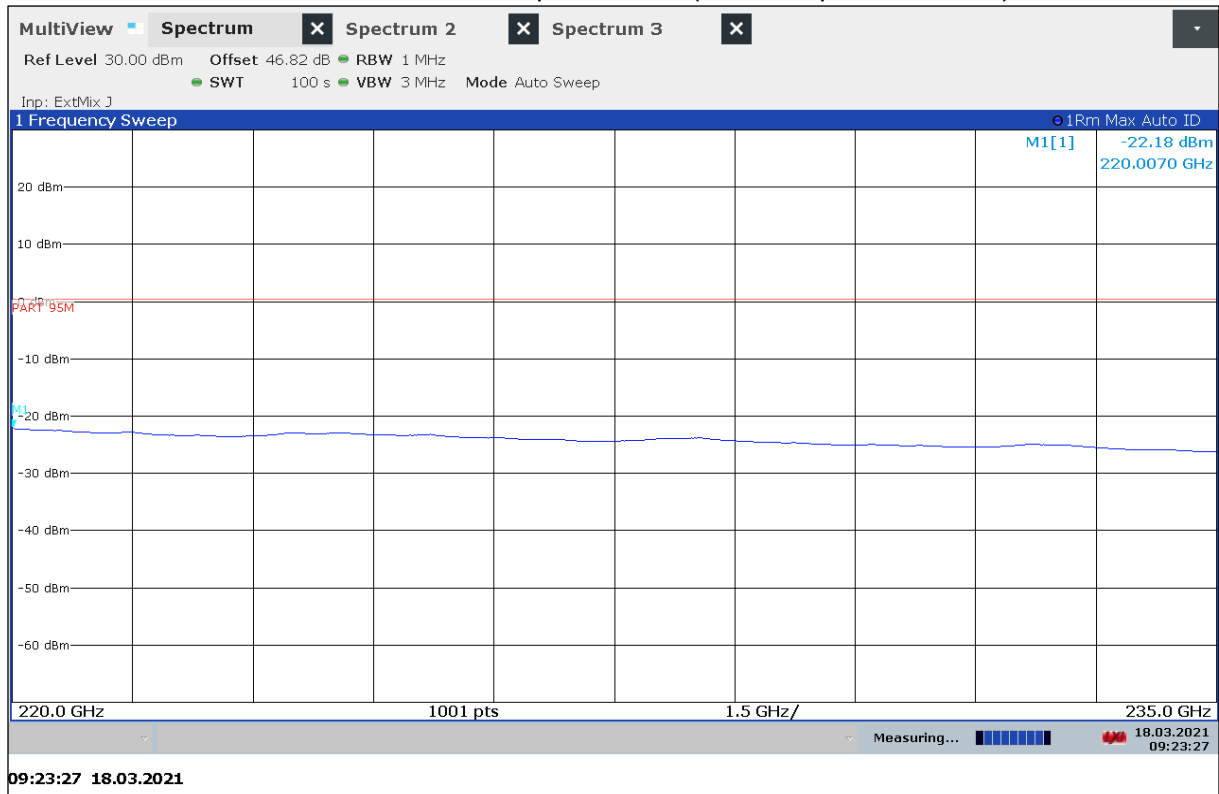
Plot 22: 220 GHz – 235 GHz, vertical / horizontal polarization, (Valid for specified Modes)
