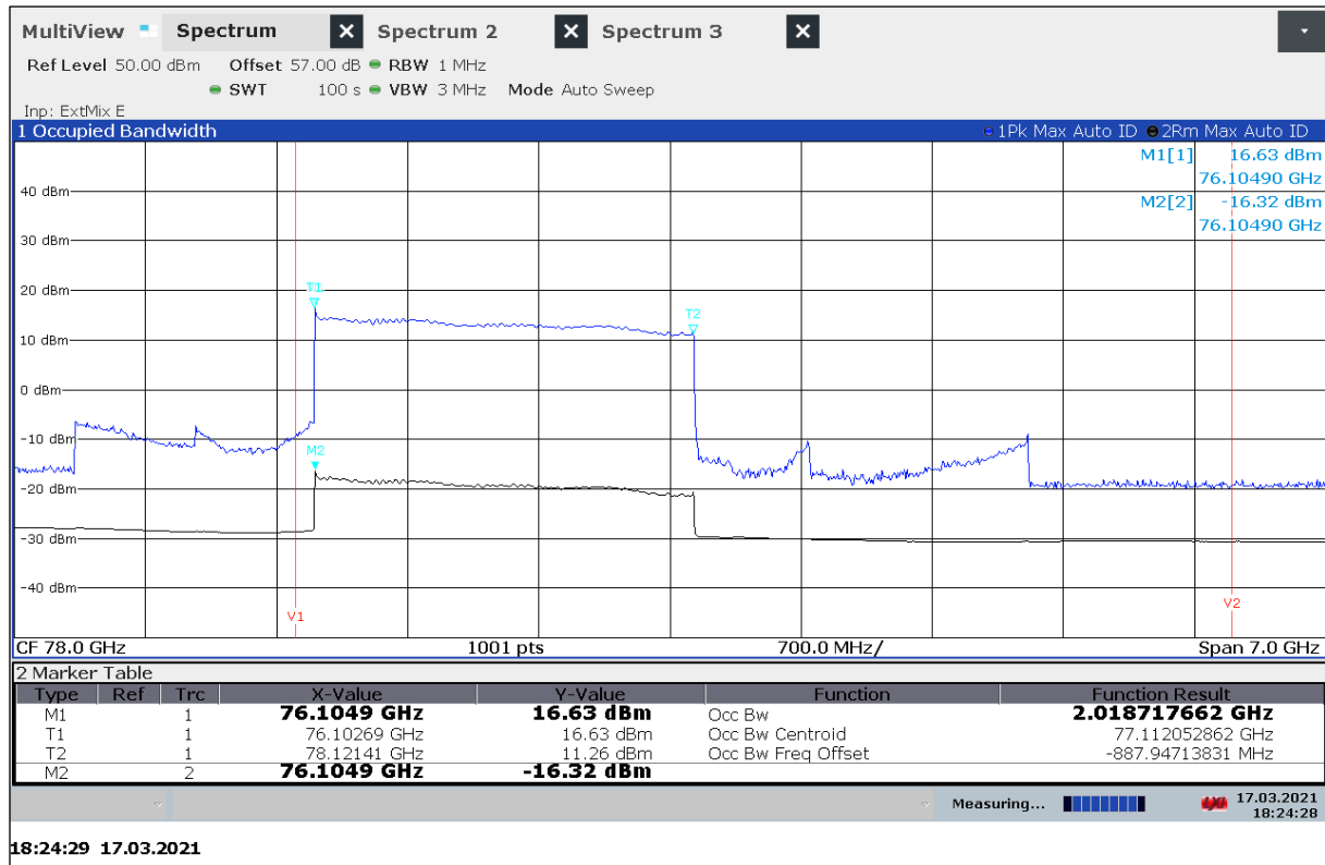
Plot 28: OBW, 30 °C / V_{nom}
