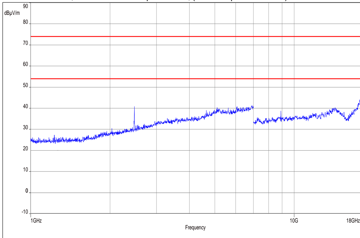
Plot 11: 1 GHz – 18 GHz, vertical / horizontal polarization, (Valid for specified Modes)
