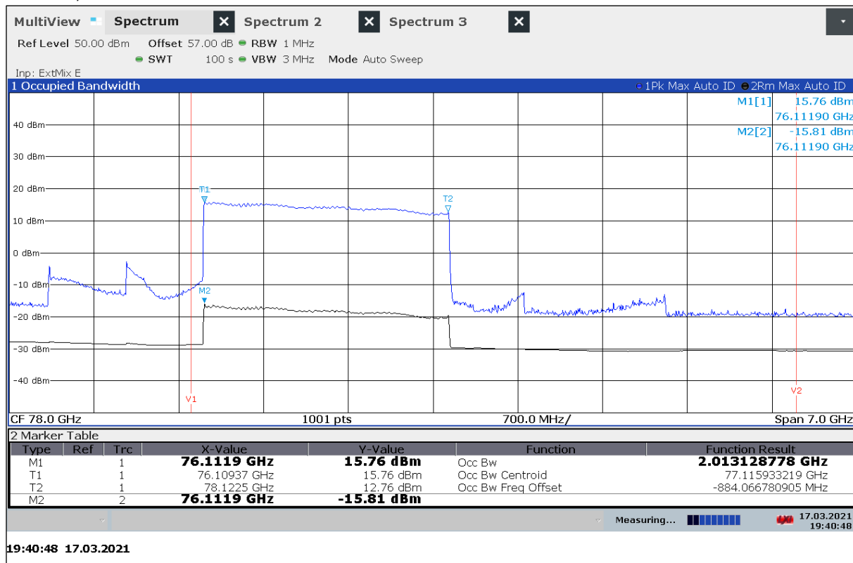
Plot 25: OBW, 0 °C / V_{nom}
