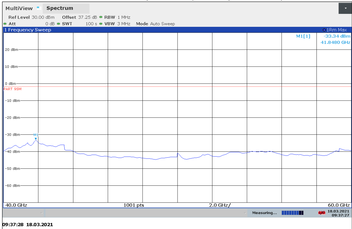
Plot 16: 40 GHz – 60 GHz, vertical / horizontal polarization, (Valid for specified Modes)
