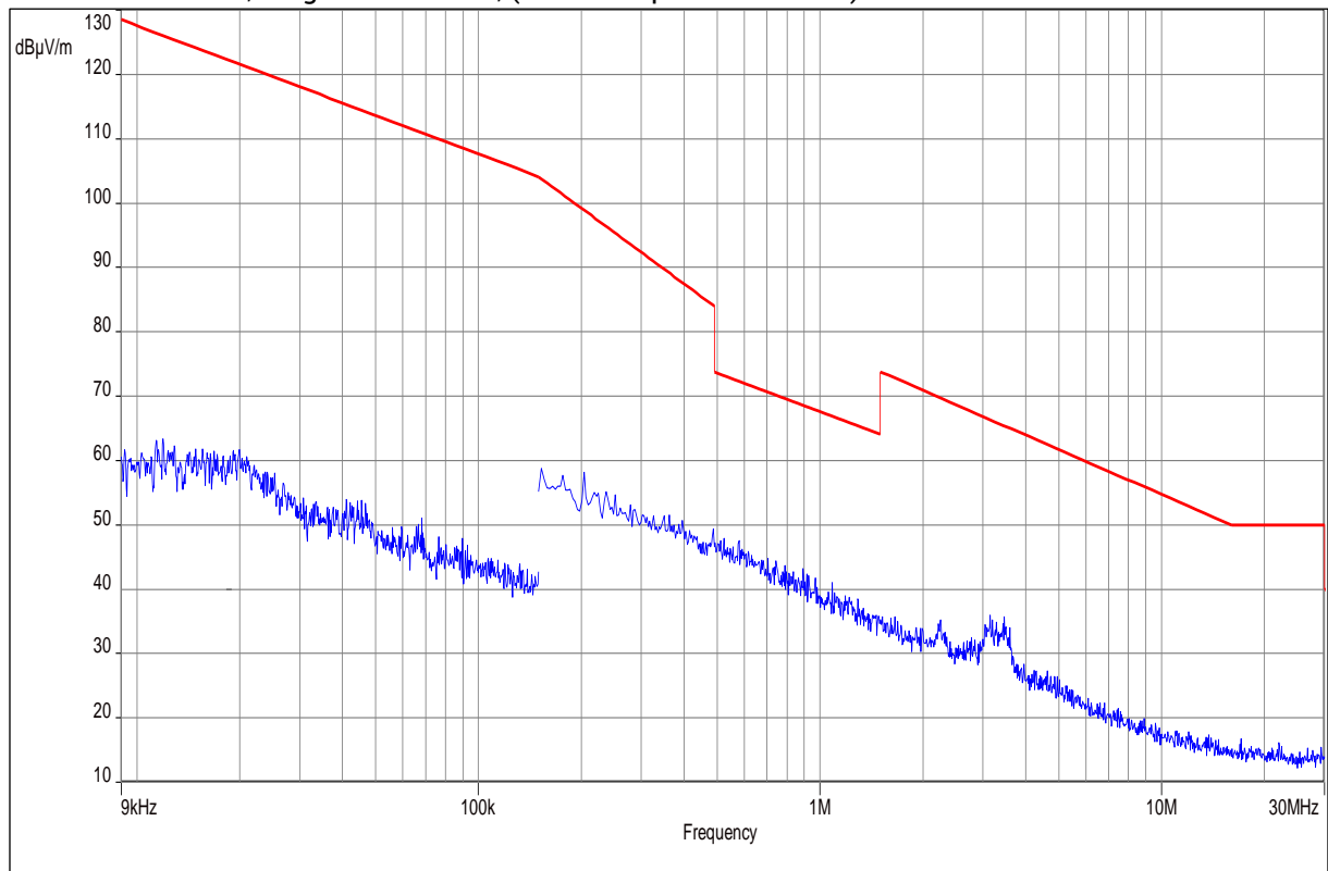
Plot 9: 9 kHz – 30 MHz, Magnetic antenna, (Valid for specified Modes)
