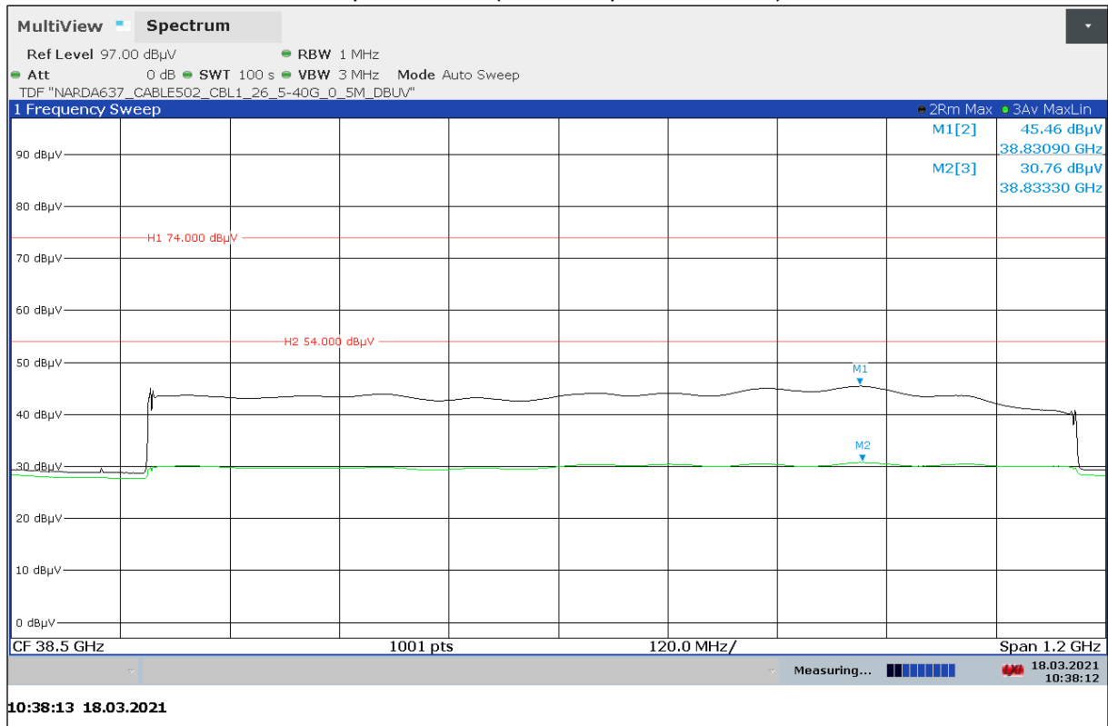
Plot 15: 38 GHz, vertical / horizontal polarization, (Valid for specified Modes)
