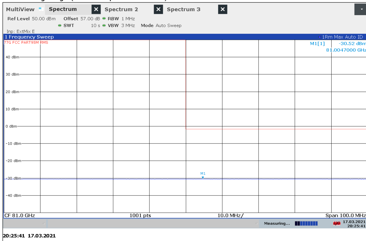
Plot 8: Band Edge High (Valid for specified Modes)
