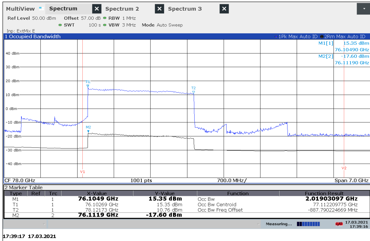
Plot 30: OBW, 50 °C / V min-max
