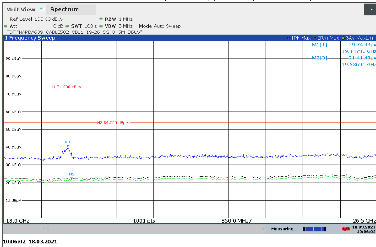
Plot 12: 18 GHz – 26.5 GHz, vertical / horizontal polarization, (Valid for specified Modes)
