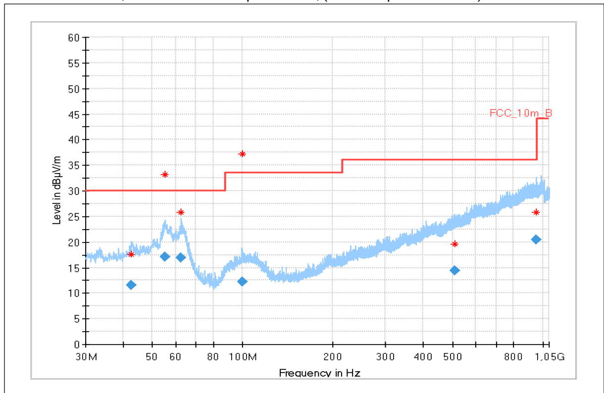
Plot 10: 30 MHz – 1 GHz, vertical / horizontal polarization, (Valid for specified Modes)
