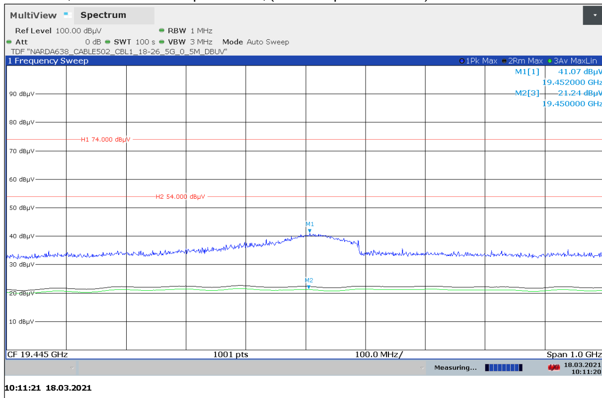
Plot 13: 19 GHz, vertical / horizontal polarization, (Valid for specified Modes)
