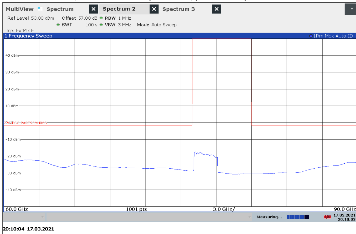
Plot 18: 60 GHz – 90 GHz, vertical / horizontal polarization, (Mode 5_5169)
