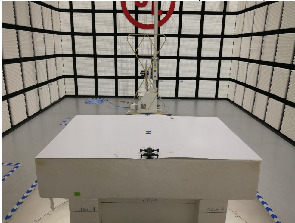
2.4G Module RADIATED RF MEASUREMENT SETUP (30MHz ~ 1 GHz)
