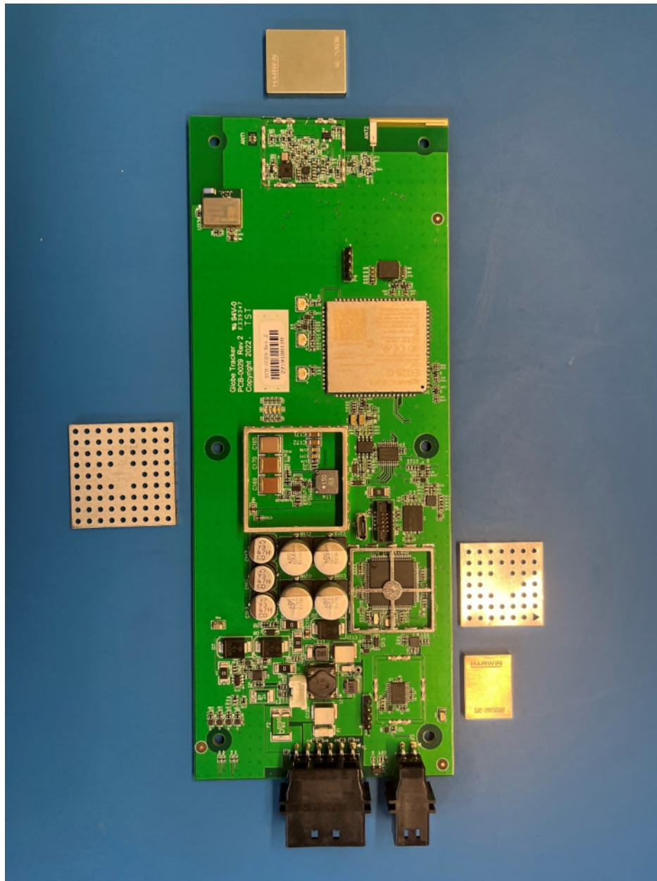
PCB Top – Shields removed
