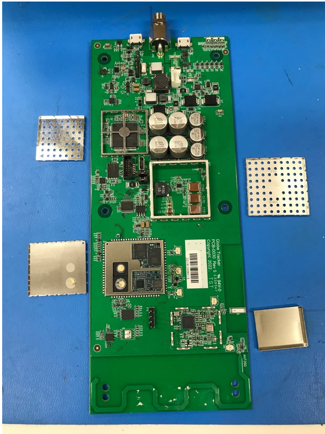
PCB Top – Shields removed
