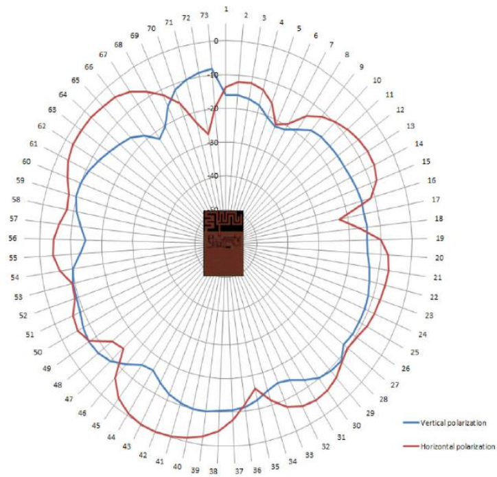
Radiation pattern, PCB horizontal, reduced size IFA, variant 2
