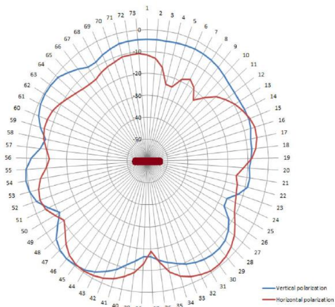
Radiation pattern, PCB vertical, reduced size IFA, variant 2
