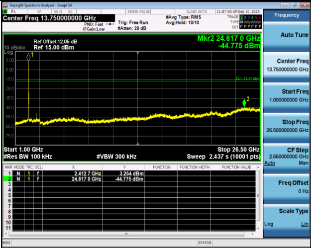
11G-Ant1-2412-1000~26500-PASS
