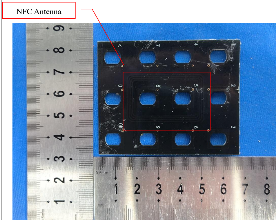
Antenna View 2
