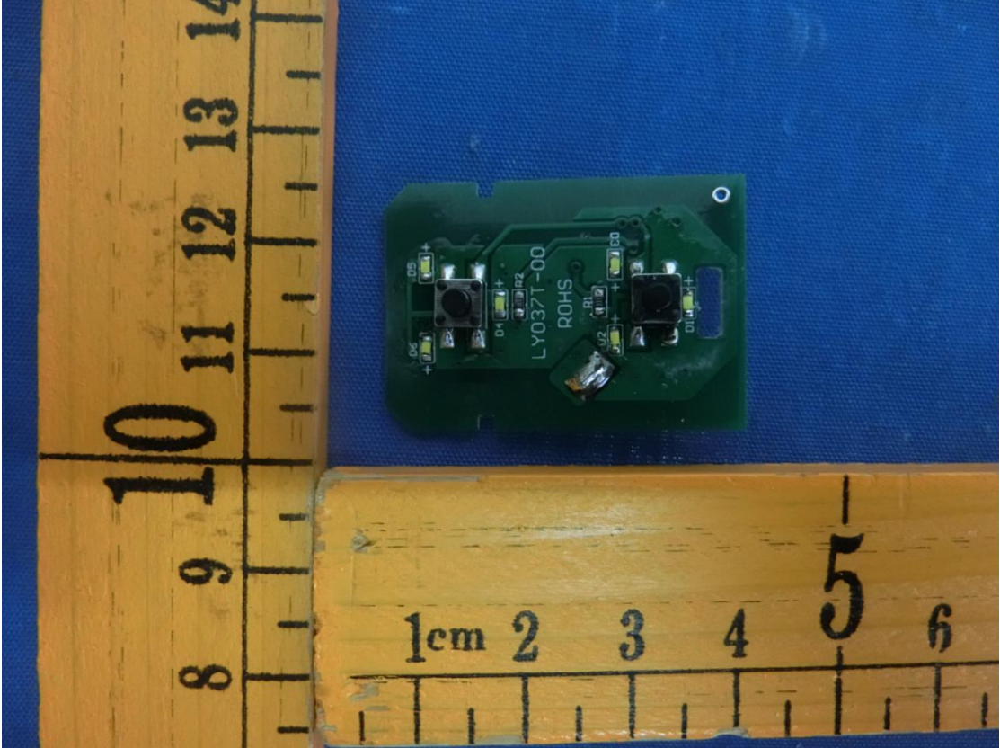
EUT - PCB View 3
