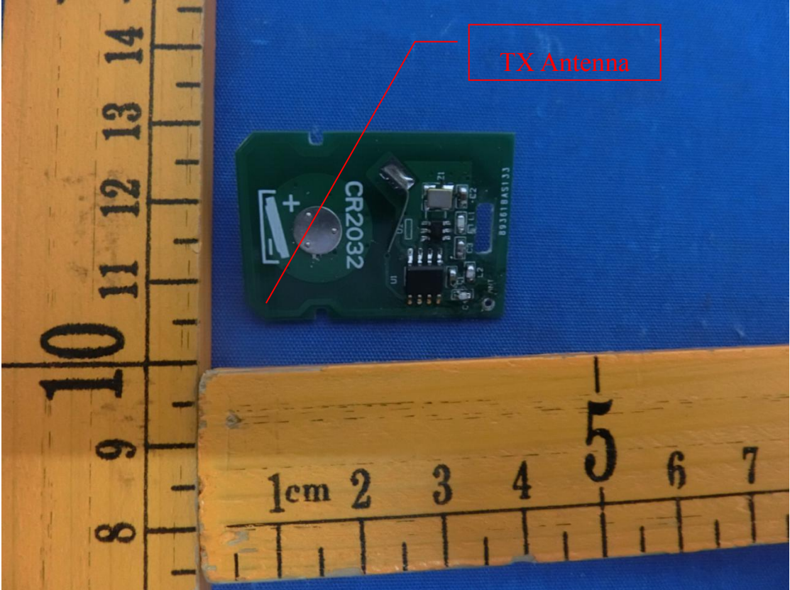
EUT – PCB View 4
