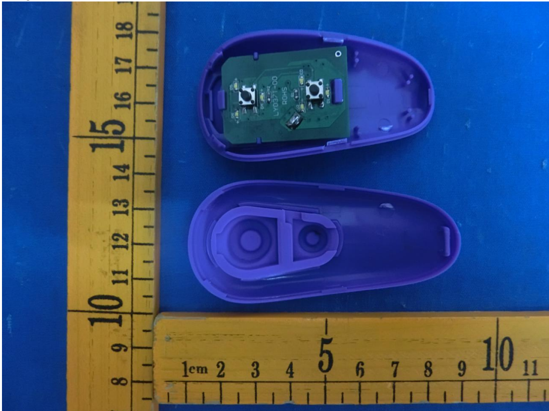
EUT - Open View 2
