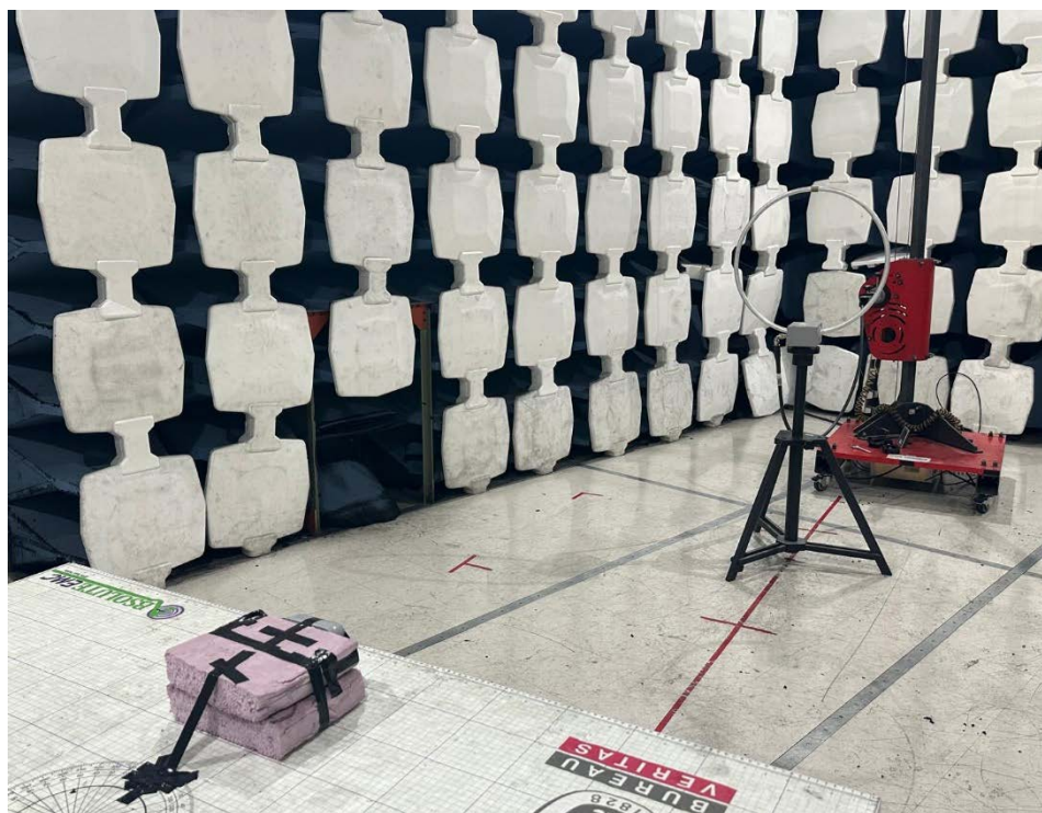
9k-30MHz Rear
