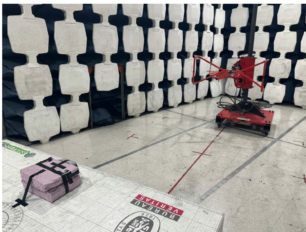
30MHz-1GHz Rear
