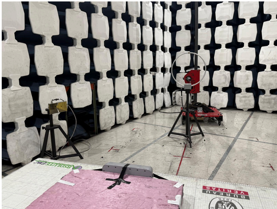
9kHz-30MHz Rear
