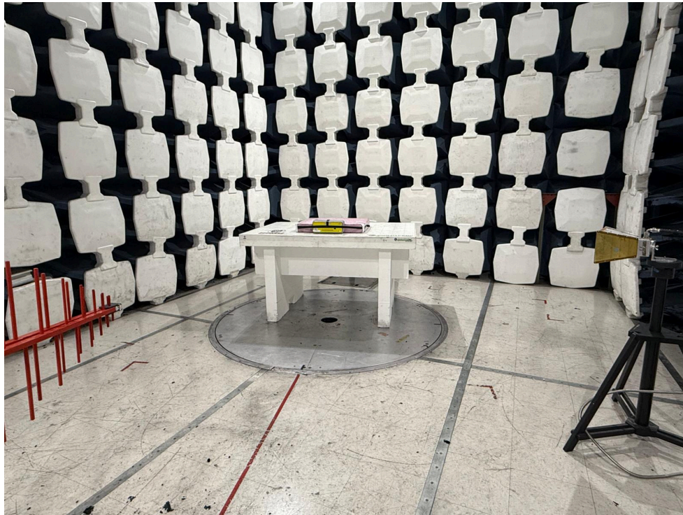
30MHz-1GHz Front
