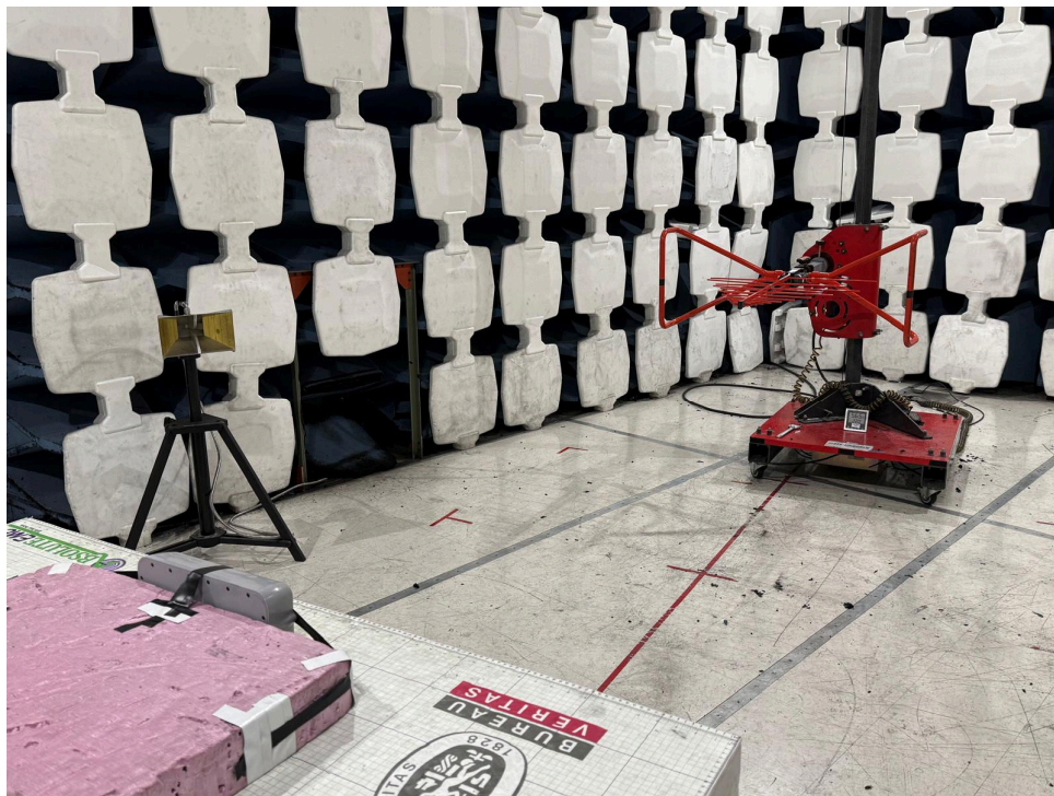
30MHz-1GHz Rear
