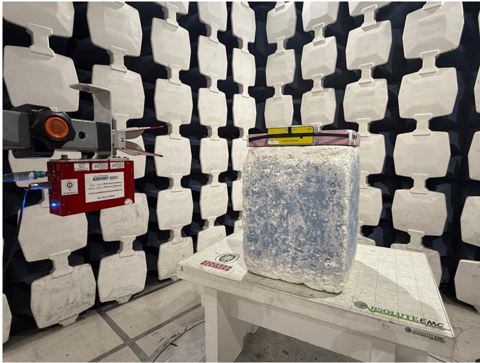
18-25GHz Front
