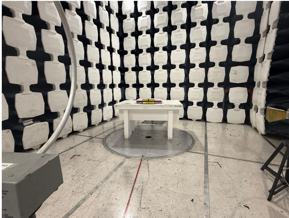
9kHz-30MHz Front
