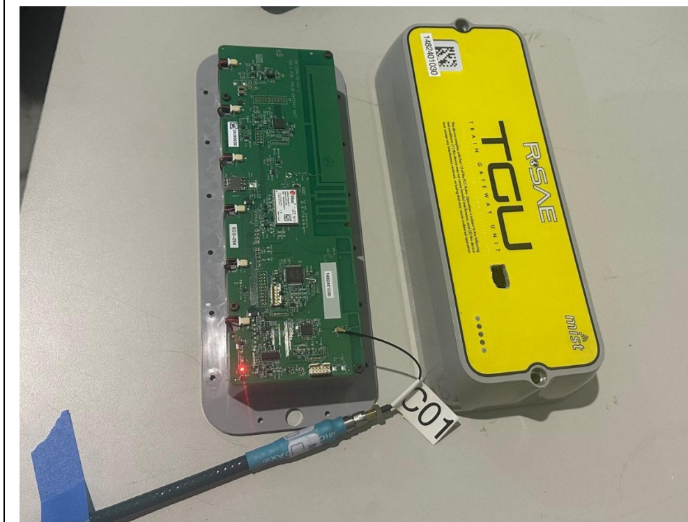
EUT Closeup
