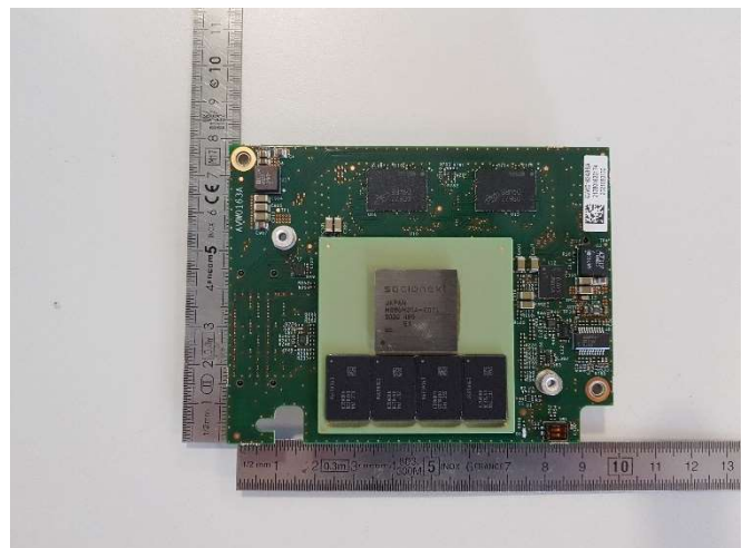
AVW0163 MENORCA Video Board
