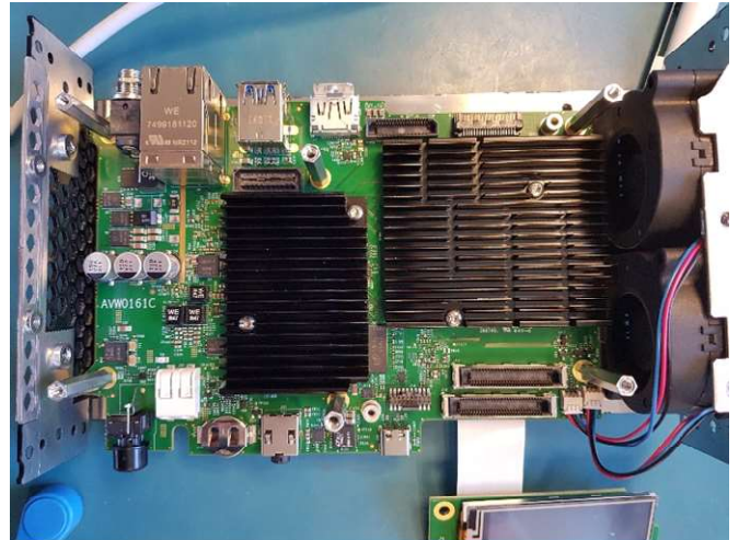
AVW0161 SIROCCO Main Board
