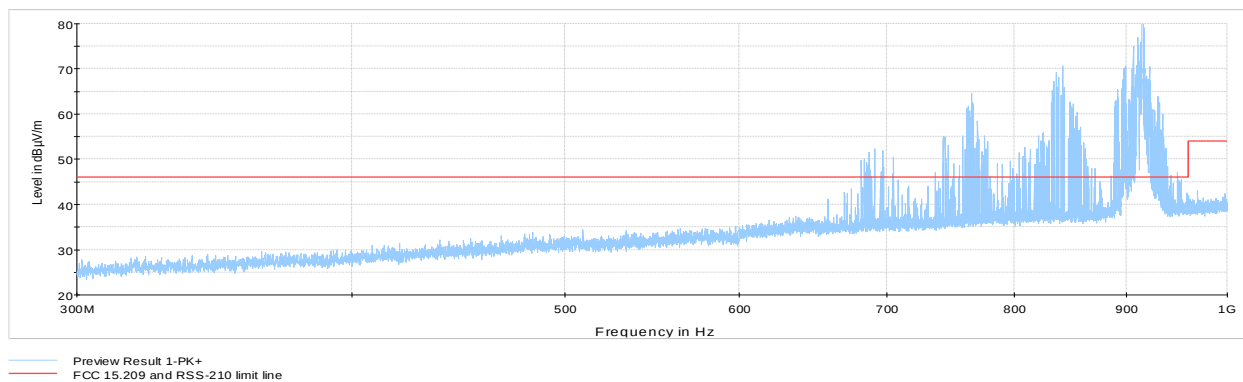
Figure 8.8-41: Radiated spurious emissions 300 MHz to 1 GHz, Tx FHSS mode mid channel with internal antenna
