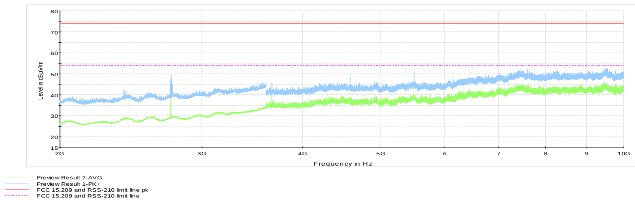
Figure 8.8-47: Radiated spurious emissions 2 GHz to 10 GHz, Tx FHSS mode mid channel with internal antenna
