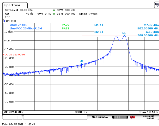
Figure 8.8-3: Conducted spurious emission at band edge, FHSS mode low channel
