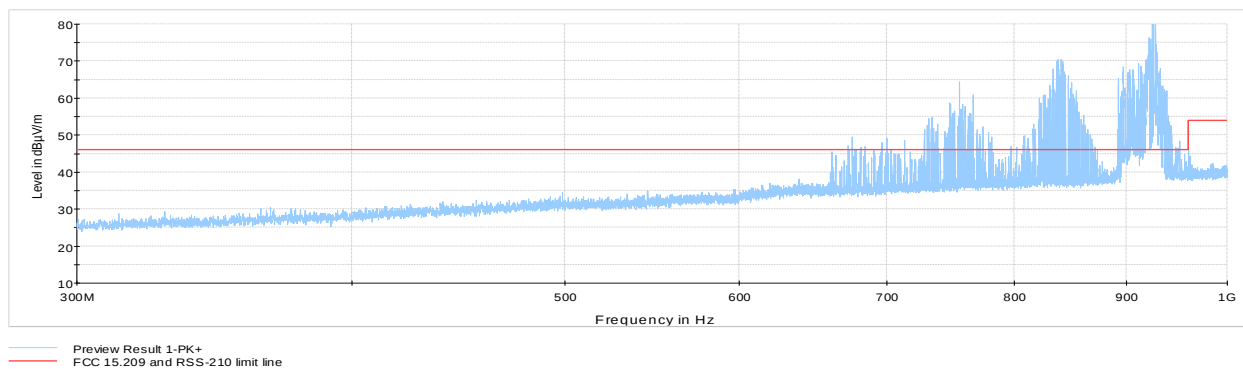
Figure 8.8-42: Radiated spurious emissions 300 MHz to 1 GHz, Tx FHSS mode hi channel with internal antenna
