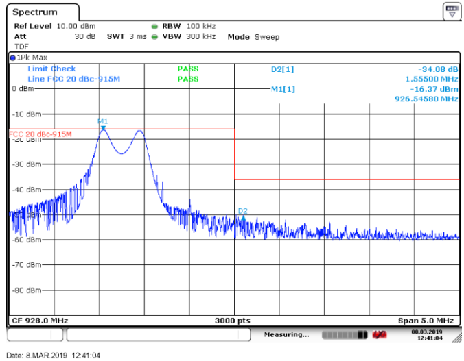
Figure 8.8-2: Conducted spurious emissions at band edge, DTS mode High channel
