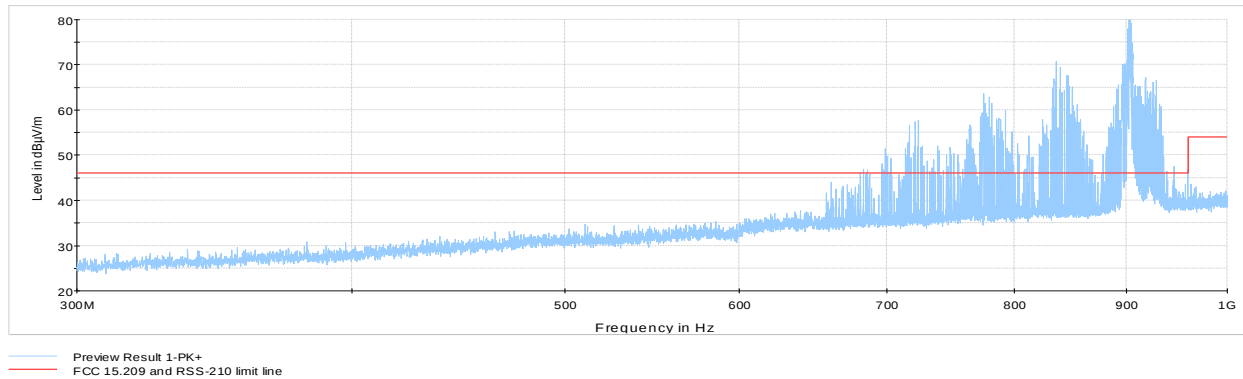
Figure 8.8-40: Radiated spurious emissions 300 MHz to 1 GHz, Tx FHSS mode Low channel with internal antenna
