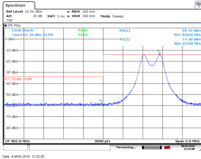
Figure 8.8-1: Conducted spurious emission at band edge, DTS mode low channel
