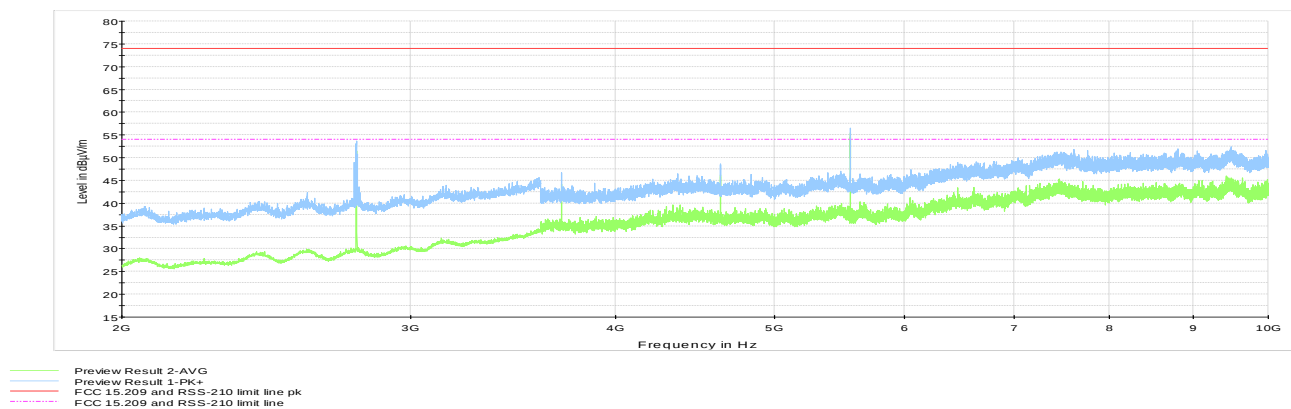
Figure 8.8-48: Radiated spurious emissions 2 GHz to 10 GHz, Tx FHSS mode hi channel with internal antenna
