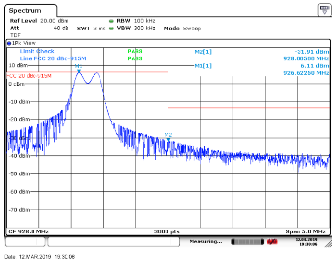
Figure 8.8-4: Conducted spurious emissions at band edge, FHSS mode High channel
