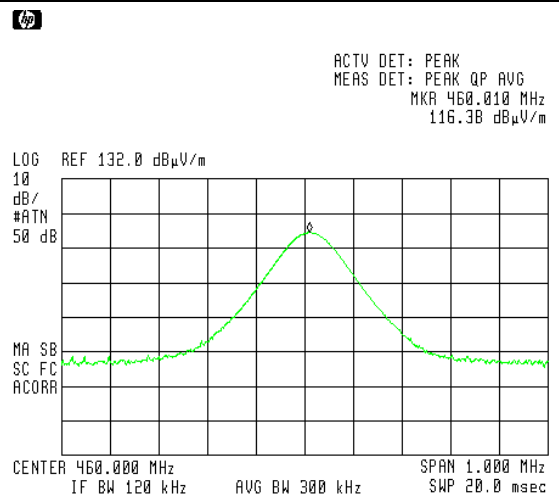
Figure 15. 460.000MHz, Horizontal
