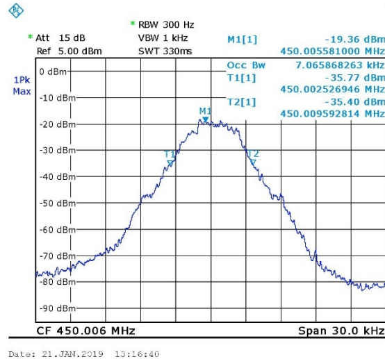
Figure 17. 450.006MHz
