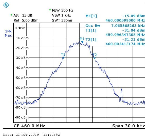
Figure 18. 460.000MHz
