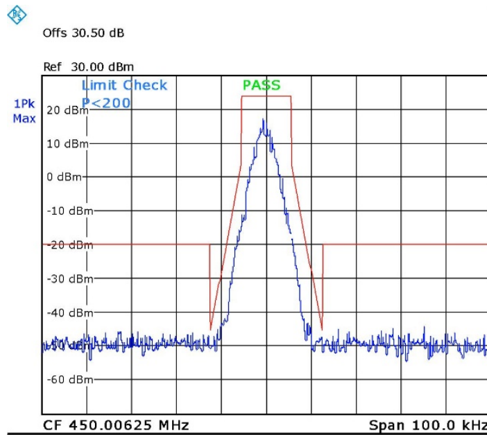
Figure 20. 450.006MHz
